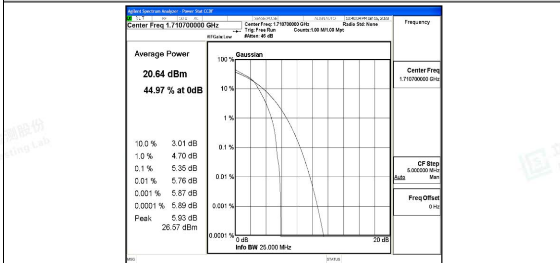
Band4-1.4MHz-16QAM-20175-6RB#0
