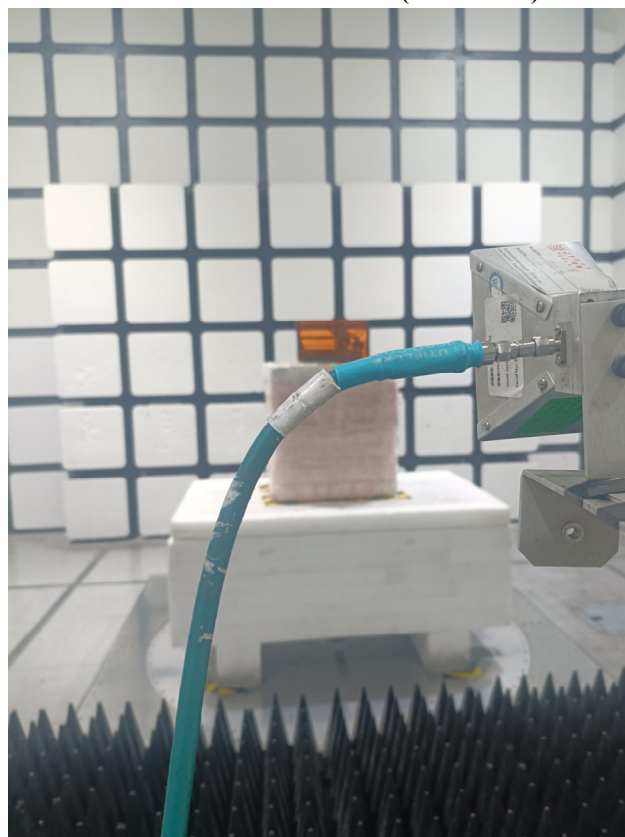
Radiated Emissions View (18-25 GHz)
