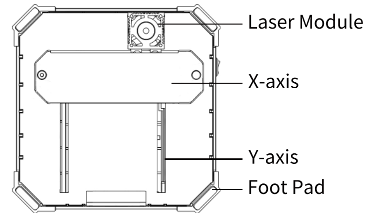
04 Bottom View
