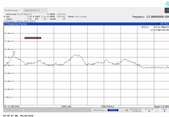
Plot 7.4.27 Radiated emission measurements at the 7 th of high carrier frequency
