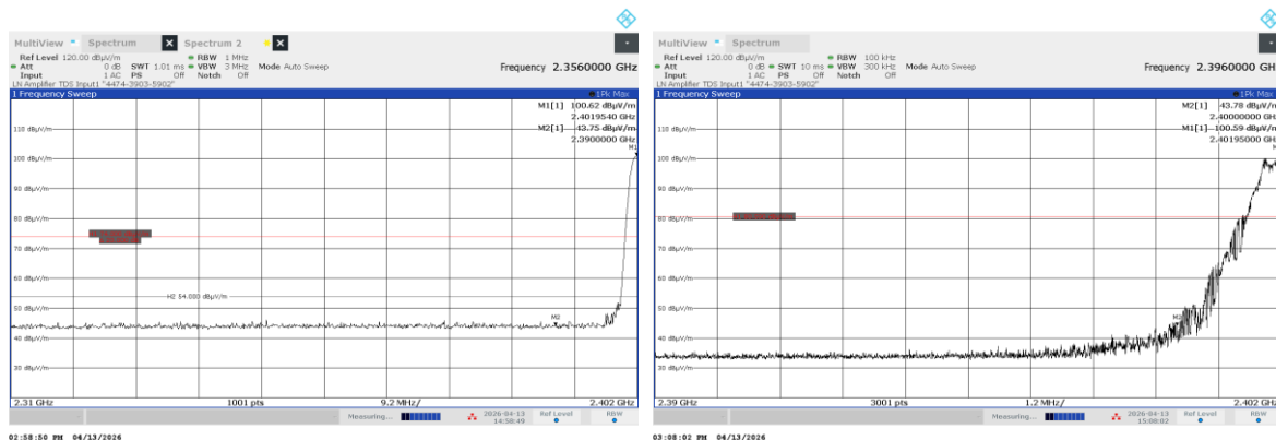
Plot 7.5.1 The highest band edge emission at low carrier frequency
