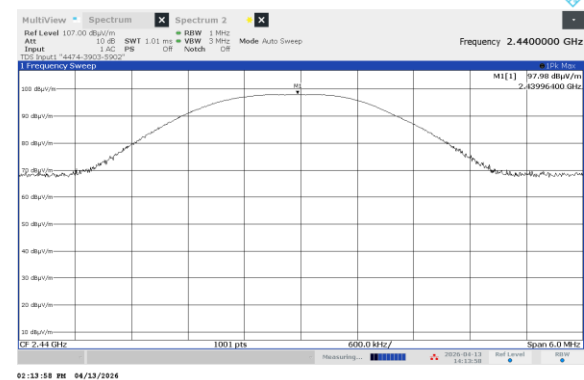
Horizontal antenna polarization
