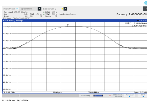
Vertical antenna polarization
