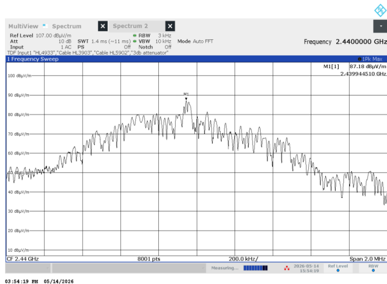
Plot 7.7.2 Peak spectral power density at mid frequency
