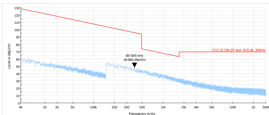
Plot 7.4.5 Radiated emission measurements from 9 kHz to 30 MHz at the mid carrier frequency
