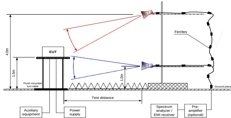
Figure 7.3.1 Setup for carrier field strength measurements
