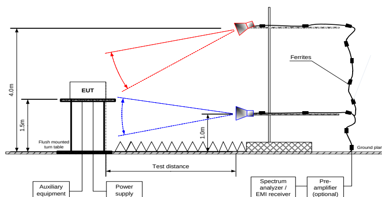
Figure 7.5.1 Band edge emission test setup
