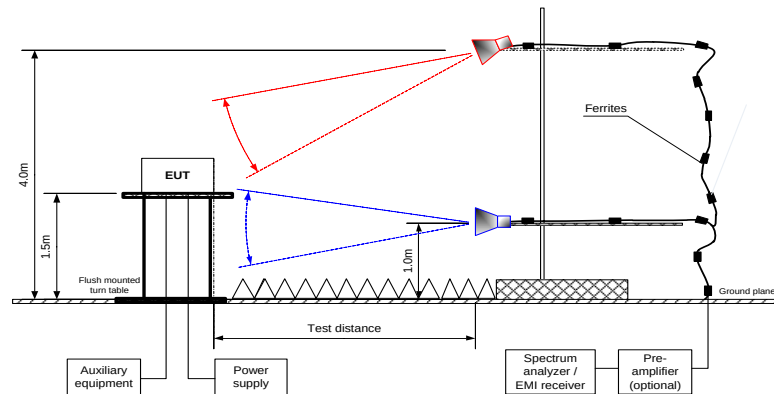
Figure 7.6.1 Setup for carrier field strength measurements
