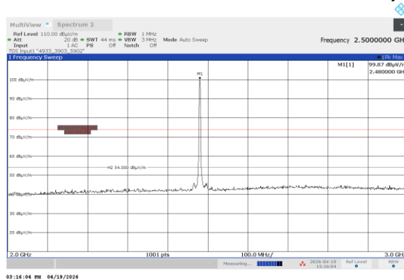
Radiated emission measurements from 2000 to 3000 MHz without Band Reject Filter 2400-2500 MHz
