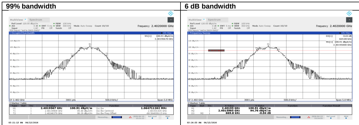
Plot 7.1.1 6 dB bandwidth test result at low frequency
