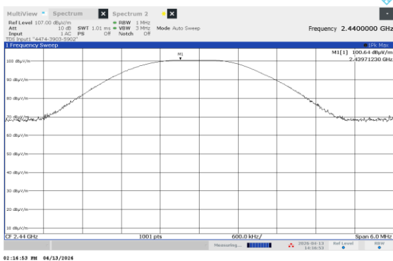
Vertical antenna polarization
