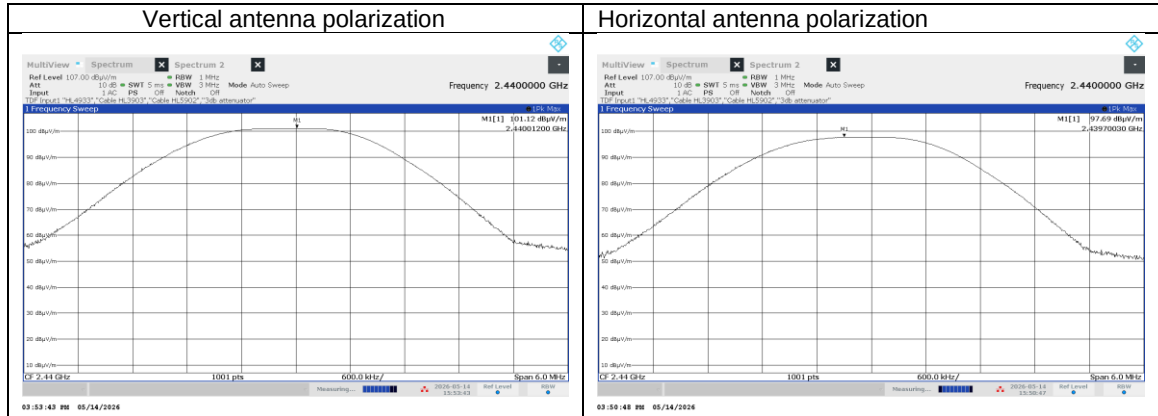
Plot 7.2.2 Field strength of carrier at mid frequency
