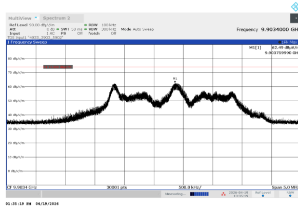
Plot 7.4.25 Radiated emission measurements at the 7 th low carrier frequency
