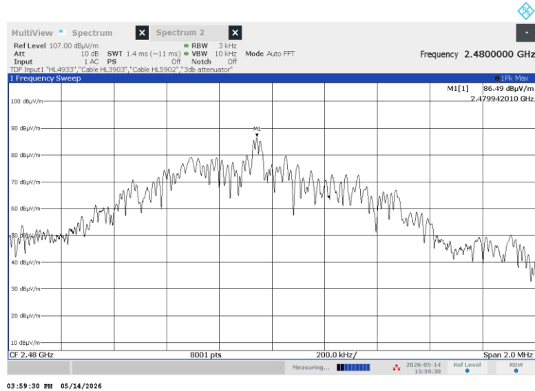
Plot 7.7.3 Peak spectral power density at high frequency
