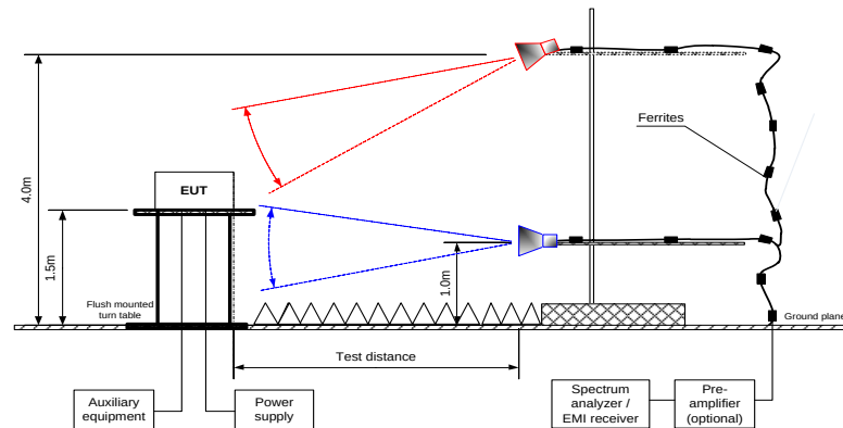
Figure 7.7.1 Setup for carrier field strength measurements
