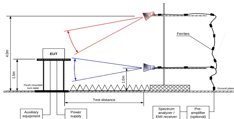
Figure 7.1.1 6 dB bandwidth test setup
