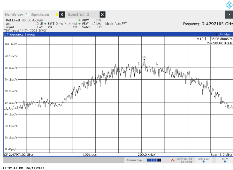
Plot 7.6.3 Peak spectral power density at high frequency
