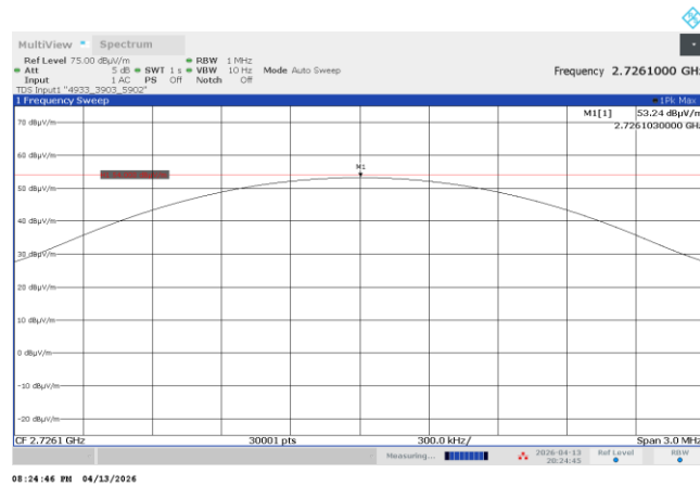
Plot 7.6.18 Radiated emission measurements at the 3 harmonic of high carrier frequency
