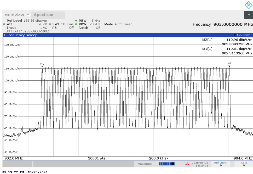
Plot 7.3.2 Number of hopping frequencies with bit rate 325 bps
