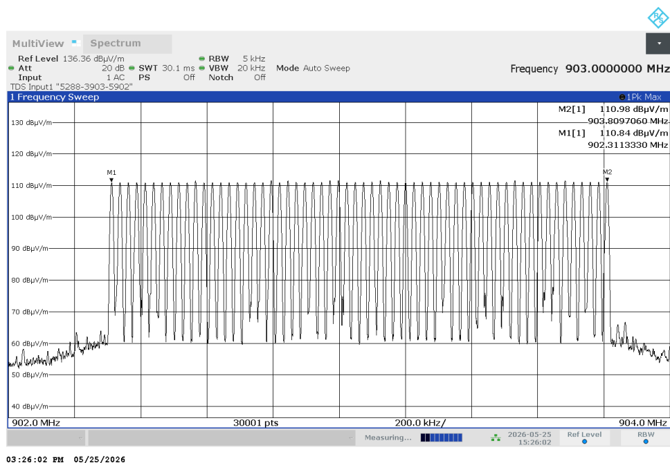
Plot 7.3.2 Number of hopping frequencies with bit rate 325 bps
