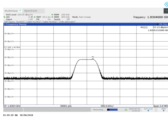
Plot 7.6.14 Radiated emission measurements at the second harmonic of mid carrier frequency
