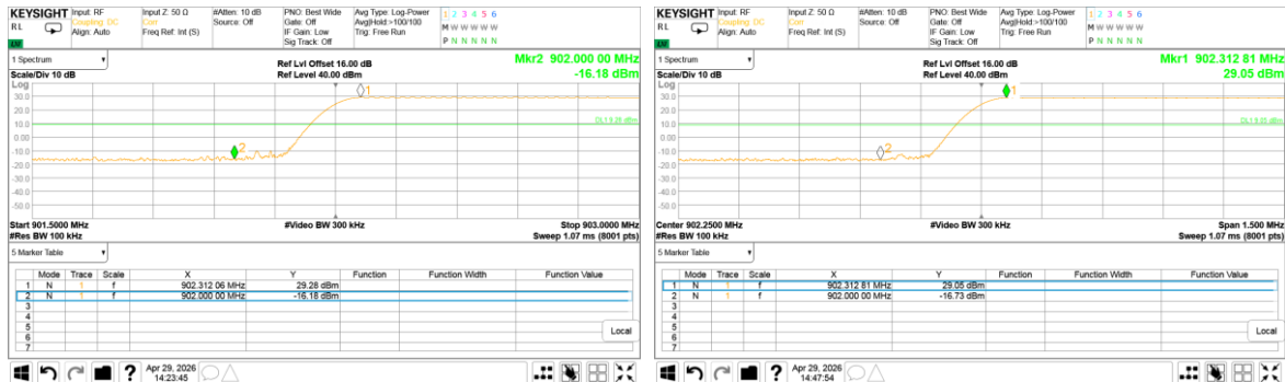
Plot 7.7.3 The highest band edge emission at low carrier frequency with hopping function enabled
