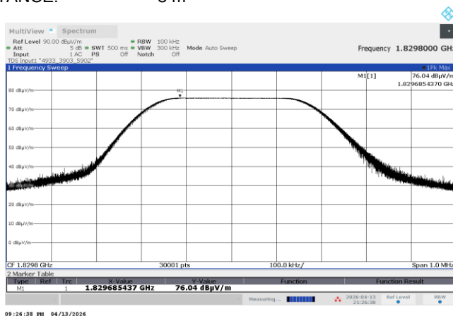
Plot 7.6.16 Radiated emission measurements at the 3 harmonic of low carrier frequency
