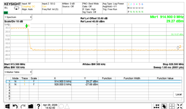
Plot 7.8.4 The highest band edge emission at high carrier frequency with hopping function enabled
