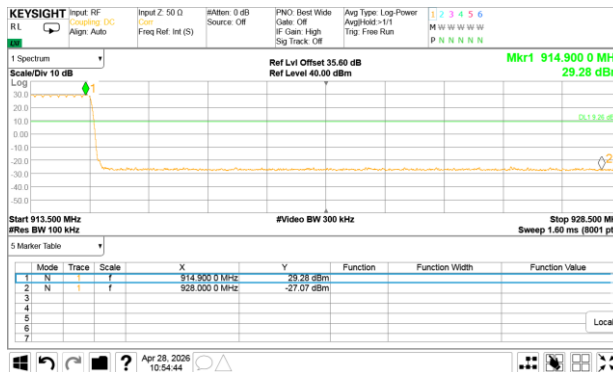
Plot 7.8.4 The highest band edge emission at high carrier frequency with hopping function enabled
