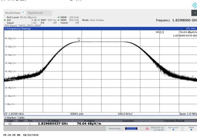
Plot 7.7.16 Radiated emission measurements at the 3 harmonic of low carrier frequency
