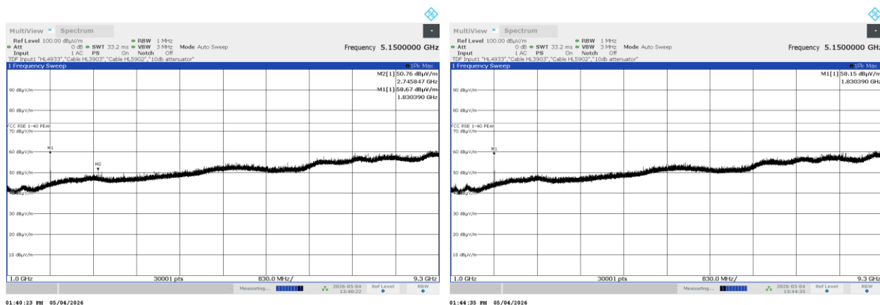
Plot 7.7.11 Radiated emission measurements from 1000 to 9500 MHz at the mid carrier frequency
