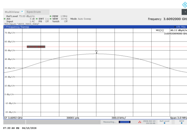
Plot 7.7.20 Radiated emission measurements at the 4 th harmonic of mid carrier frequency
