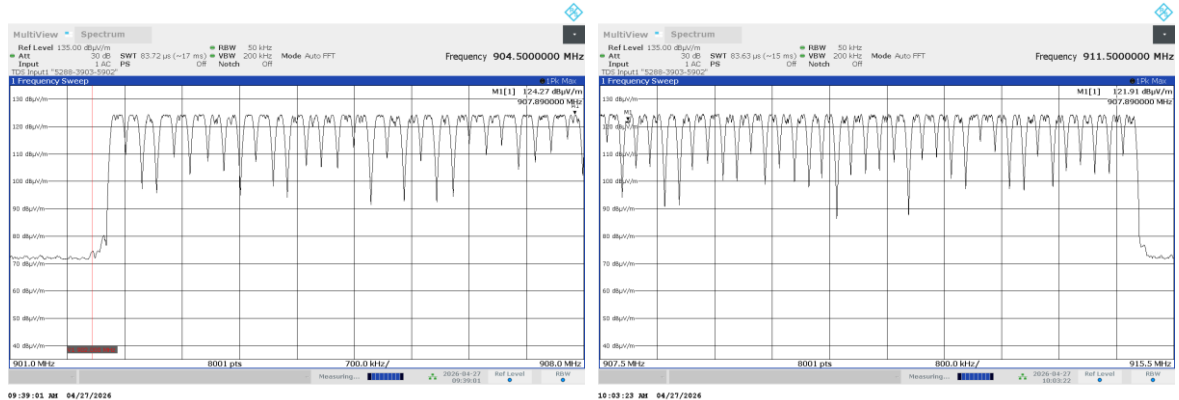
Plot 7.3.1 Number of hopping frequencies with bit rate 250 bps
