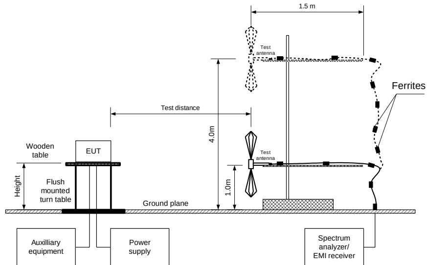
Figure 7.8.1 Band edge emission test setup (hopping disables)
