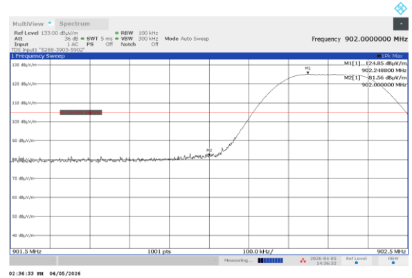
Plot 7.8.1 The highest band edge emission at low carrier frequency with hopping function disabled
