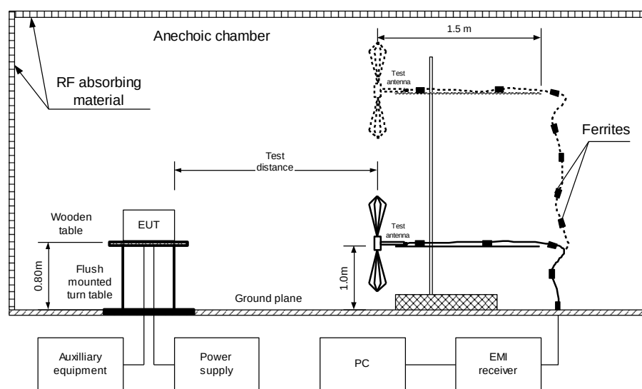
Figure 7.3.1 Hopping frequencies test setup
