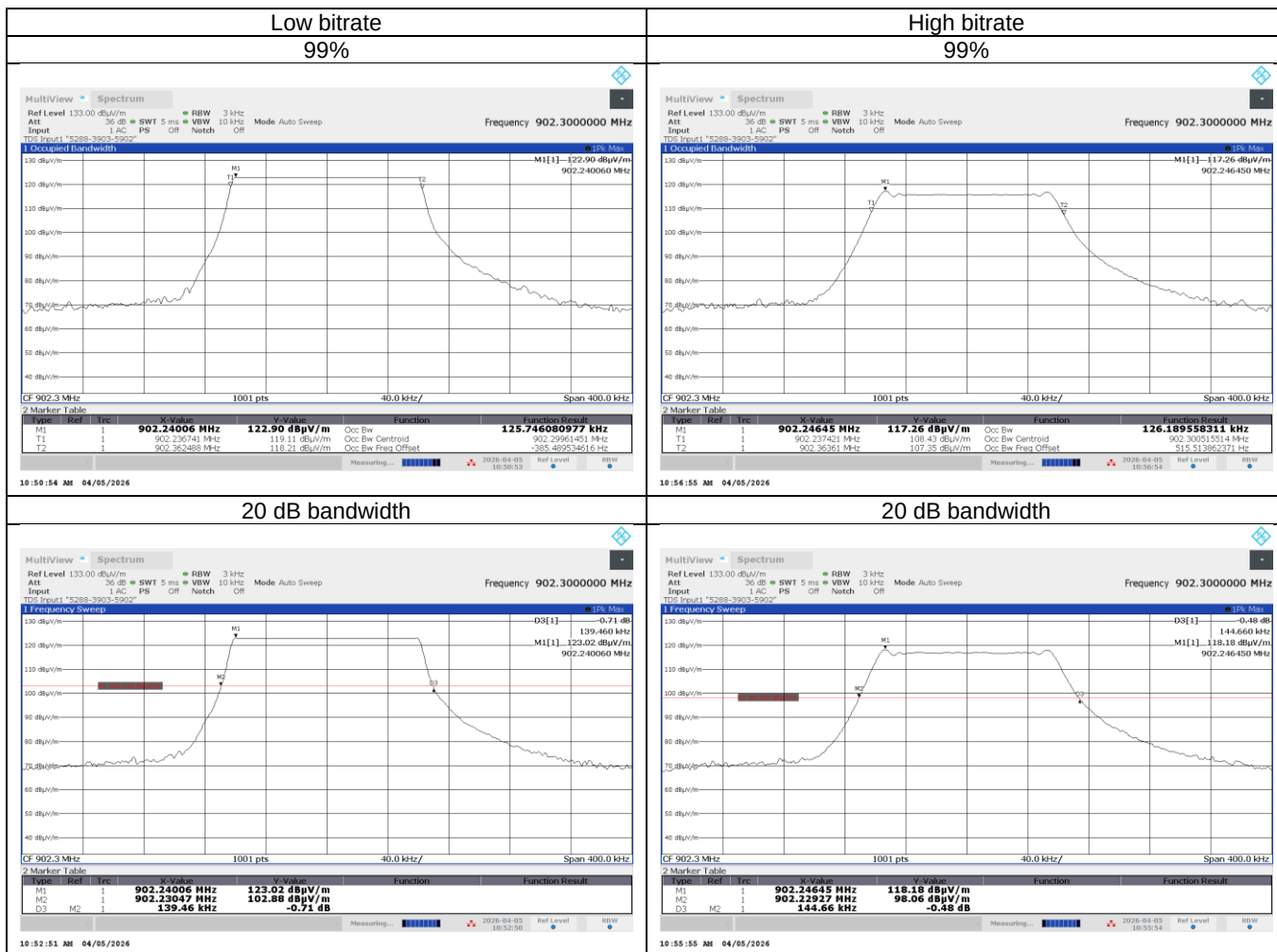
Plot 7.1.1 20 dB bandwidth test result at low frequency
