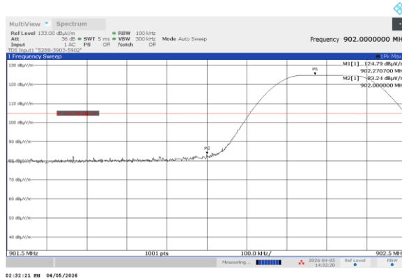
Plot 7.8.1 The highest band edge emission at low carrier frequency with hopping function disabled
