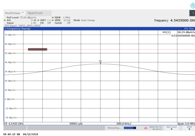
Plot 7.7.24 Radiated emission measurements at the 6 th harmonic of high carrier frequency
