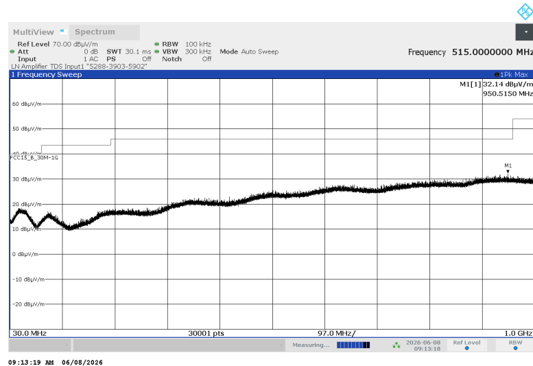
Plot 7.3.8 Radiated emission measurements from 30 to 1000 MHz at the mid carrier frequency
