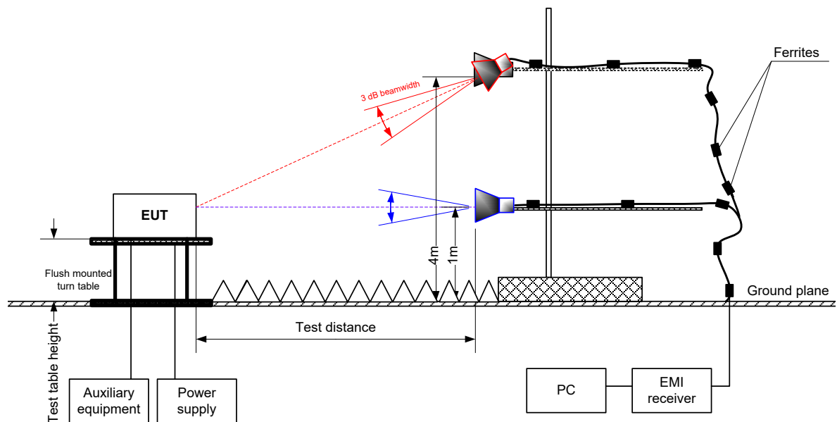
Figure 8.1.2 Setup for radiated emission measurements in semi anechoic chamber in 1000 – 12500 MHz range, table-top EUT
