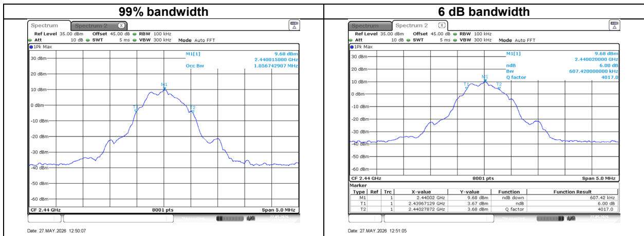
Plot 7.1.2 6 dB bandwidth test result at mid frequency
