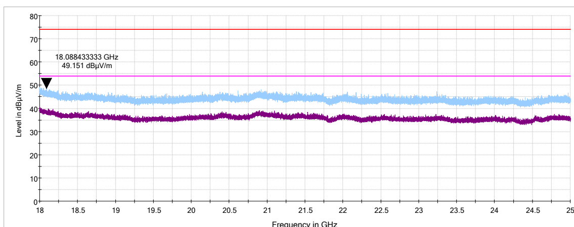
Plot 7.3.14 Radiated emission measurements from 18000 to 25000 MHz at the mid carrier frequency
