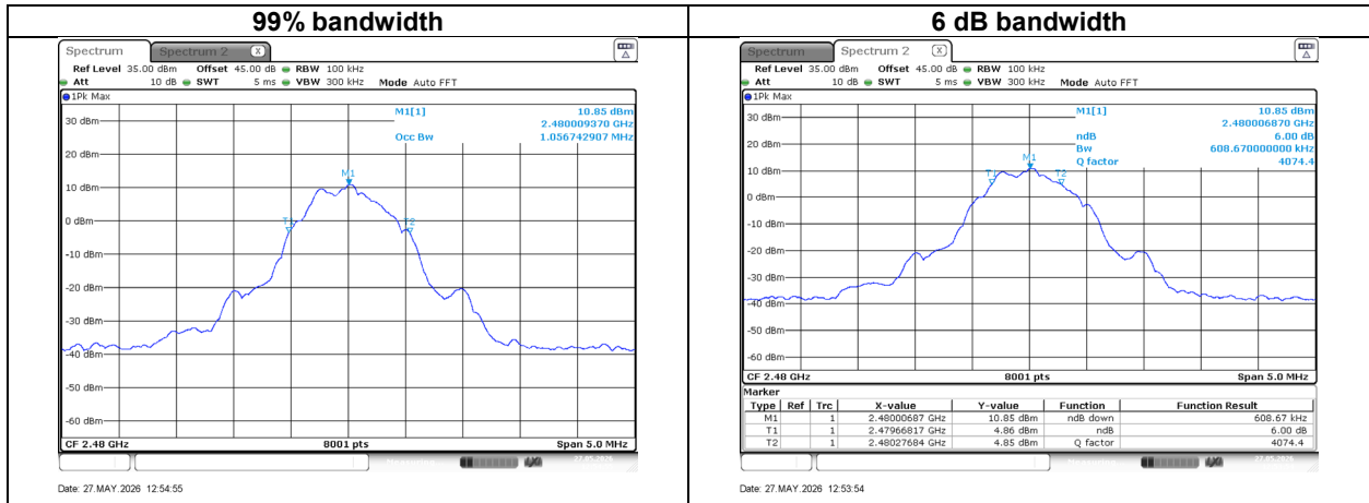
Plot 7.1.3 6 dB bandwidth test result at high frequency
