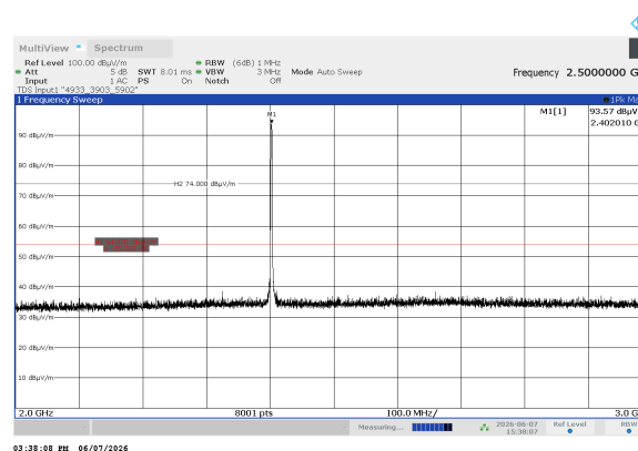
Radiated emission measurements from 2000 to 3000 MHz without Reject Band Filter HL 4338
