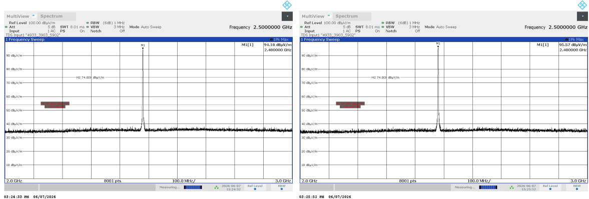
Radiated emission measurements from 2000 to 3000 MHz without Reject Band Filter HL 4338
