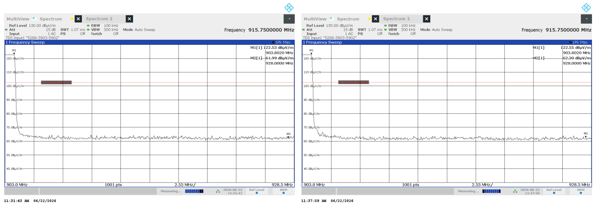
Plot 7.7.4 The highest band edge emission at high carrier frequency with hopping function enabled
