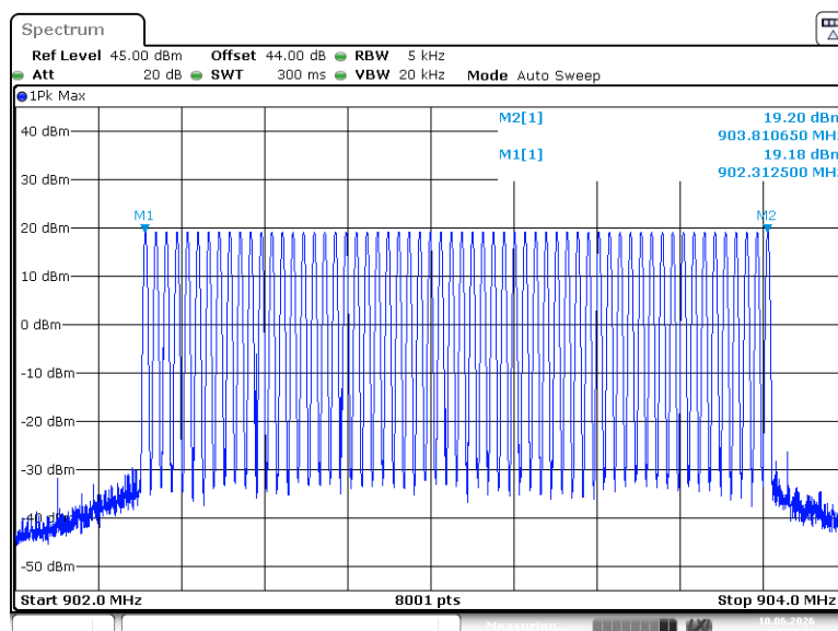
Plot 7.3.2 Number of hopping frequencies with bit rate 325 bps
