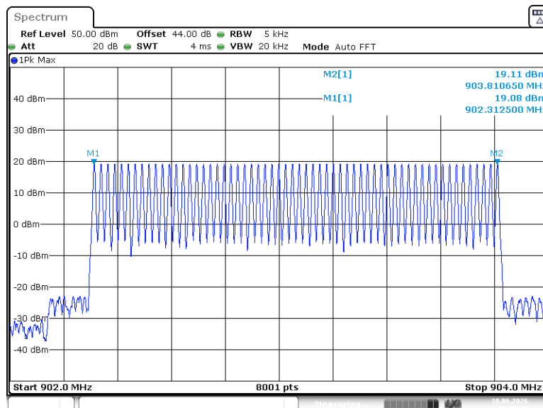
Plot 7.3.1 Number of hopping frequencies with bit rate 162 bps
