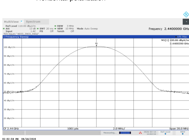
Plot 7.4.5 Field strength of carrier at mid frequency at AT98-7-23-11-S-5-N
