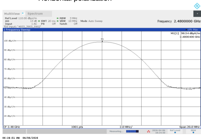
Plot 7.4.3 Field strength of carrier at high frequency at AT98-7-2-21-S-5-N
