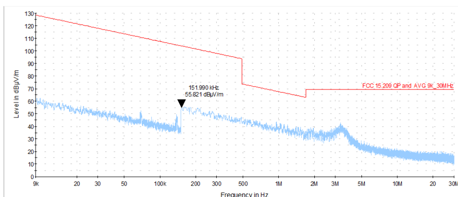
Plot 7.6.5 Radiated emission measurements from 9 kHz to 30 MHz at the mid carrier frequency
