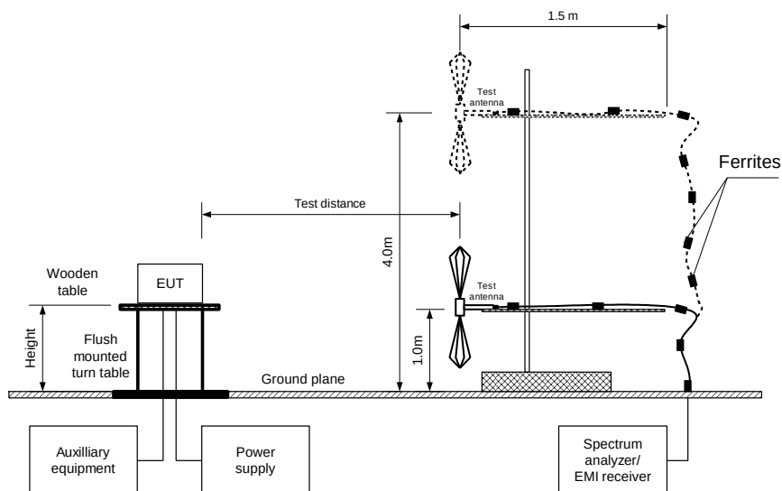
Figure 7.5.2 Setup for spurious emission field strength measurements in 30 -1000 MHz
