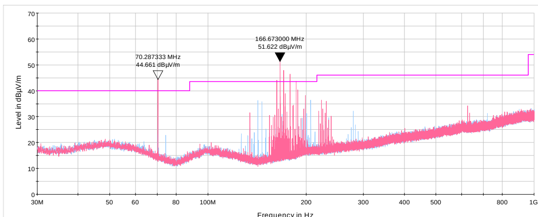
Plot 7.5.8 Radiated emission measurements from 30 to 1000 MHz at the mid carrier frequency
