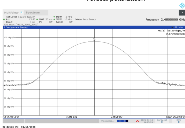
Plot 7.4.6 Field strength of carrier at high frequency at AT98-7-23-11-S-5-N
