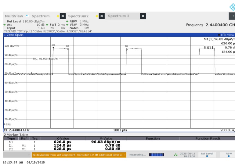
Plot 7.5.16 Transmission pulse duration and period
