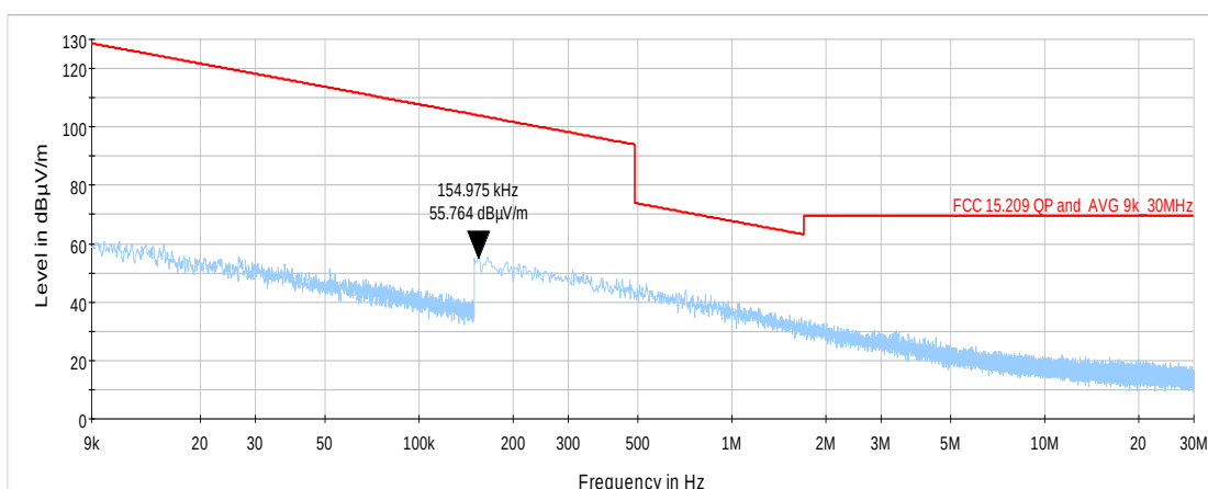
Plot 7.5.5 Radiated emission measurements from 9 kHz to 30 MHz at the mid carrier frequency
