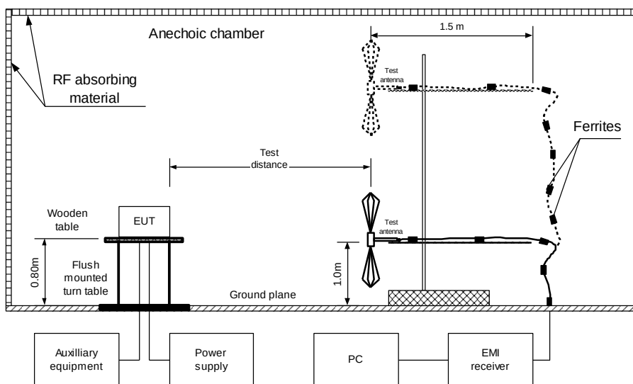
Figure 8.2.1 Setup for radiated emission measurements in anechoic chamber in 30 – 1000 MHz range, table-top EUT
