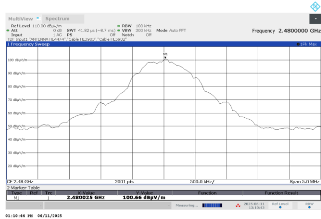
Plot 7.5.3 Peak spectral power density at high frequency
