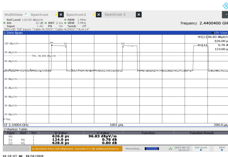
Plot 7.3.49 Transmission pulse duration and period
