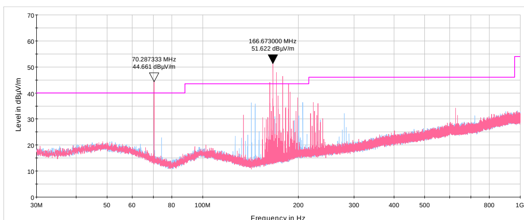
Plot 7.3.8 Radiated emission measurements from 30 to 1000 MHz at the mid carrier frequency
