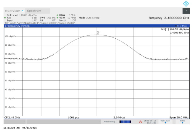
Plot 7.2.6 Field strength of carrier at high frequency at AT98-7-2-11-S-5-N
