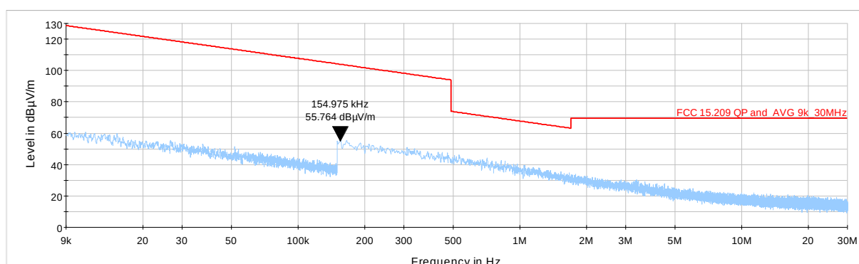
Plot 7.3.5 Radiated emission measurements from 9 kHz to 30 MHz at the mid carrier frequency
