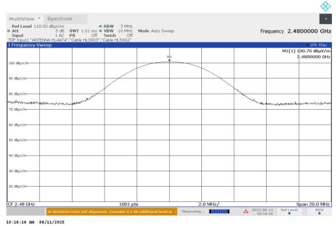
Plot 7.2.3 Field strength of carrier at high frequency at AT98-7-23-17-S-5-N
