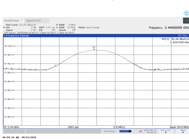
Plot 7.2.2 Field strength of carrier at mid frequency at AT98-7-23-17-S-5-N
