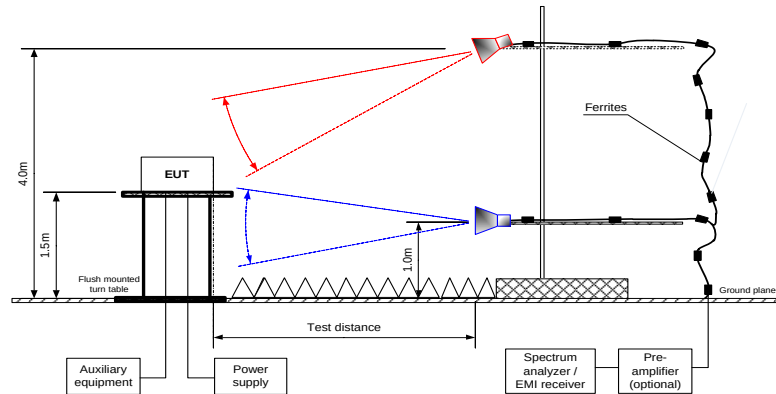
Figure 7.5.1 Setup for carrier field strength measurements
