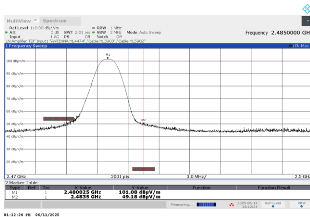
Plot 7.6.2 The highest band edge emission at high carrier frequency
