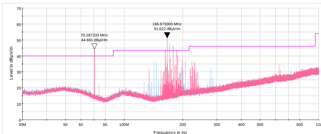
Plot 7.4.8 Radiated emission measurements from 30 to 1000 MHz at the mid carrier frequency
