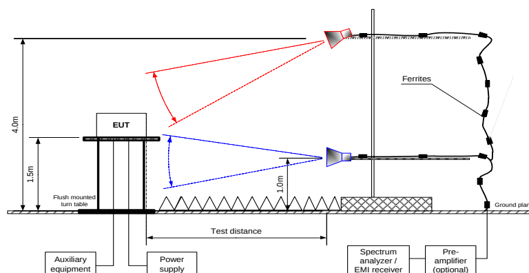
Figure 7.7.1 Band edge emission test setup
