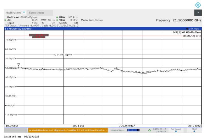
Plot 7.4.14 Radiated emission measurements from 18000 to 25000 MHz at the mid carrier frequency
