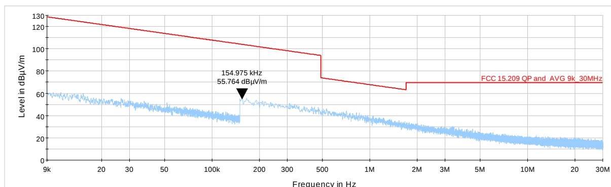
Plot 7.4.5 Radiated emission measurements from 9 kHz to 30 MHz at the mid carrier frequency
