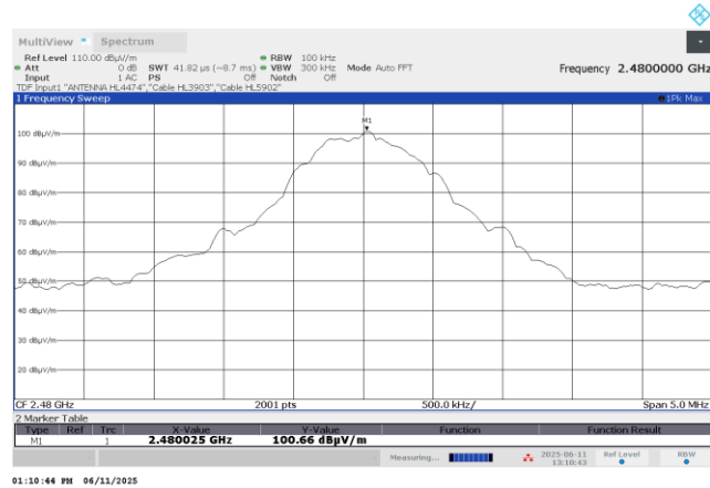
Plot 7.8.3 Peak spectral power density at high frequency
