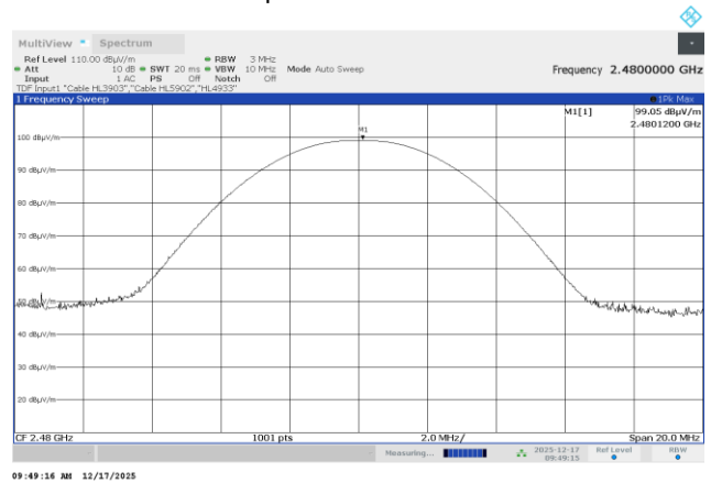
Plot 7.3.3 Field strength of carrier at high frequency at AT98-1-13-P-5-N
