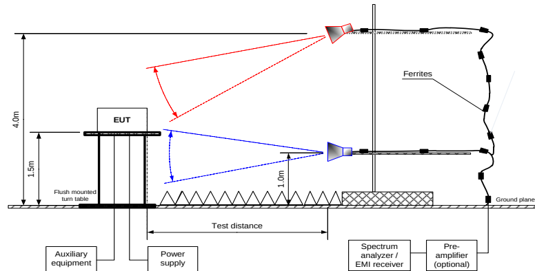
Figure 7.8.1 Setup for carrier field strength measurements
