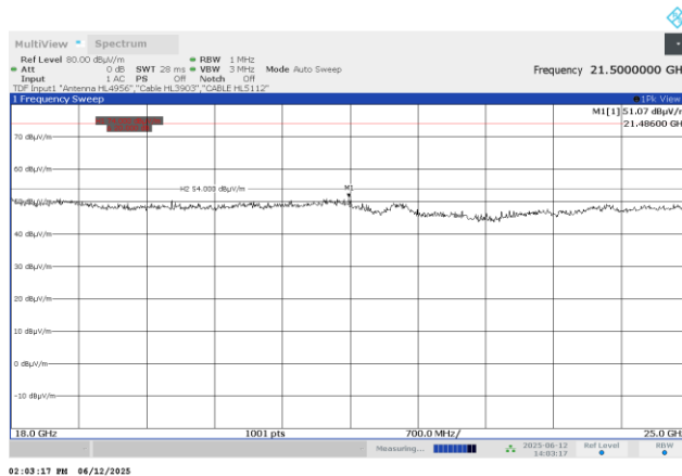
Plot 7.4.14 Radiated emission measurements from 18000 to 25000 MHz at the mid carrier frequency
