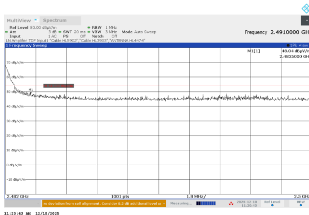
Plot 7.7.2 The highest band edge emission at high carrier frequency
