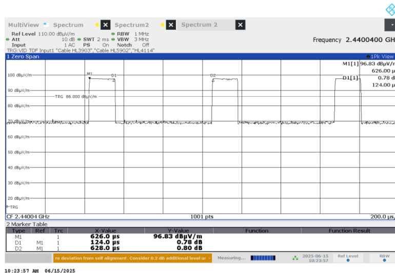
Plot 7.4.16 Transmission pulse duration and period
