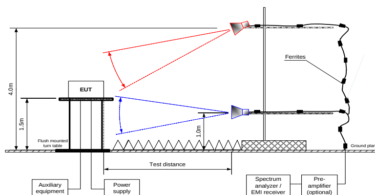
Figure 7.6.1 Band edge emission test setup
