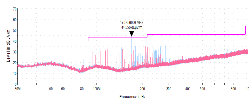
Plot 7.5.8 Radiated emission measurements from 30 to 1000 MHz at the mid carrier frequency
