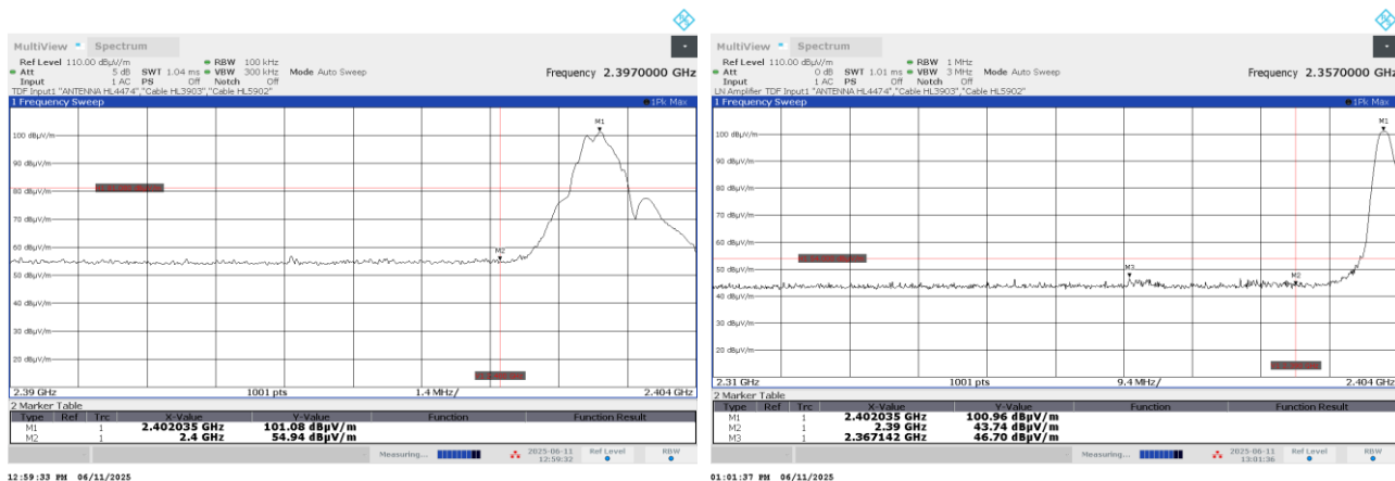
Plot 7.6.1 The highest band edge emission at low carrier frequency
