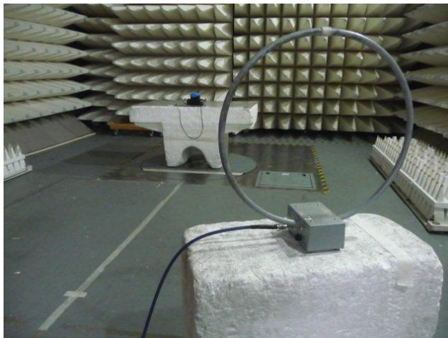
Photograph No.1 Setup for spurious emission field strength measurements in the anechoic chamber below 30 MHz for Digital water meter
