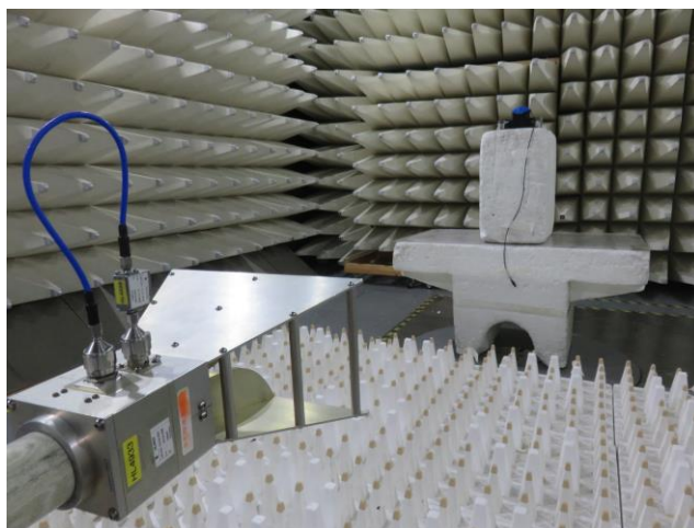
Photograph No.4 Setup for spurious emission field strength measurements in the anechoic chamber in 18-40 GHz range for Digital water meter
