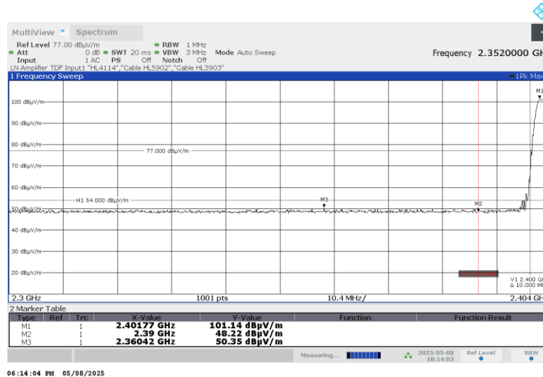
Plot 7.8.2 The highest emission level within the assigned band at high carrier frequency
