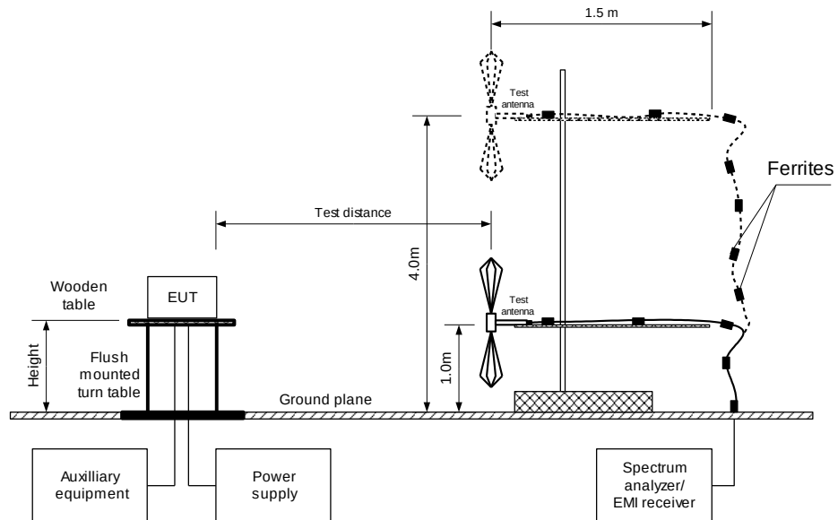
Figure 7.9.1 Setup for carrier field strength measurements
