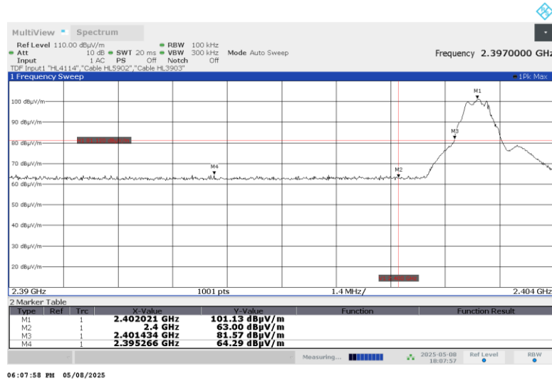
Plot 7.8.3 The highest band edge emission at low carrier frequency
