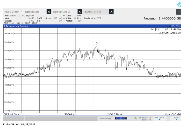
Plot 7.9.2 Peak spectral power density at mid frequency
