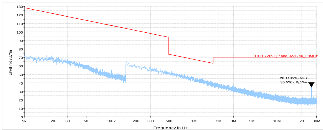
Plot 7.8.5 Radiated emission measurements from 0.009 to 30 MHz at the mid carrier frequency
