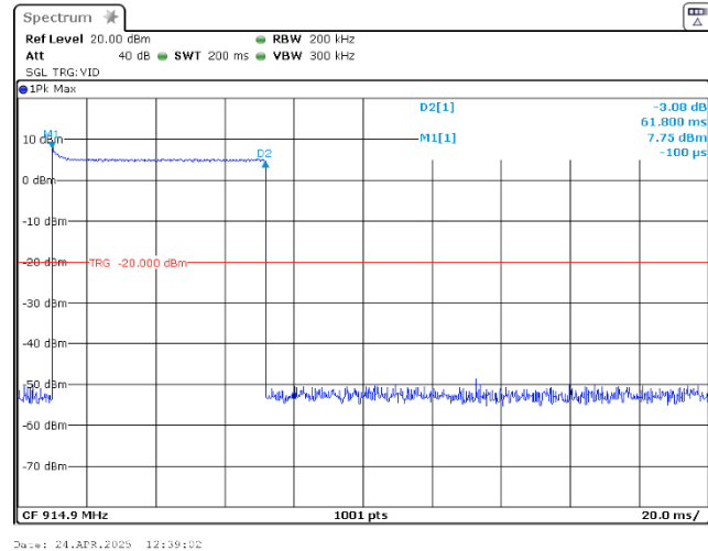
Plot 7.8.16 Transmission pulse duration
