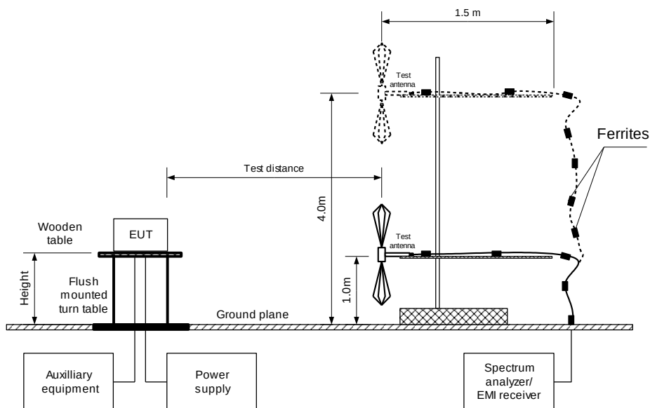
Figure 7.9.2 Setup for spurious emission field strength measurements from 30 to 1000 MHz
