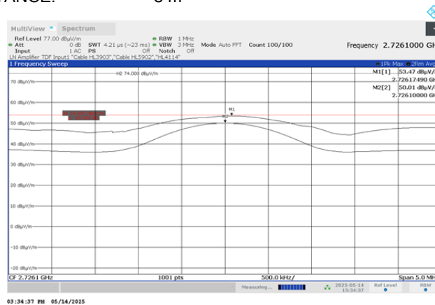
Plot 7.8.15 Radiated emission measurements at the third harmonic of high carrier frequency
