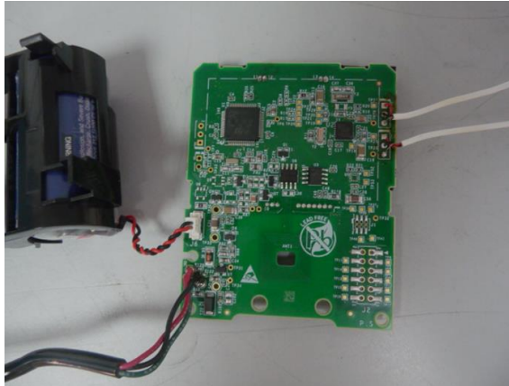
Photograph No.1 Sonata Sprint 2 - general front internal view
