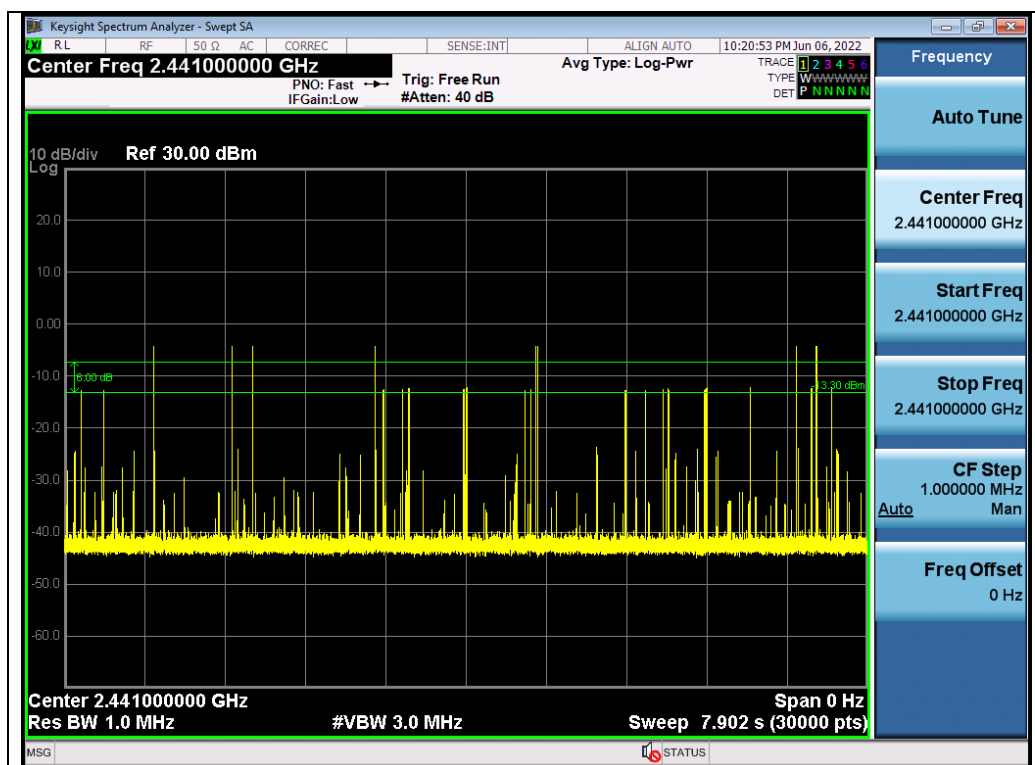
Test Graph BR HOP ANT1 NA 1Mbps 2441 Number of Busrt
