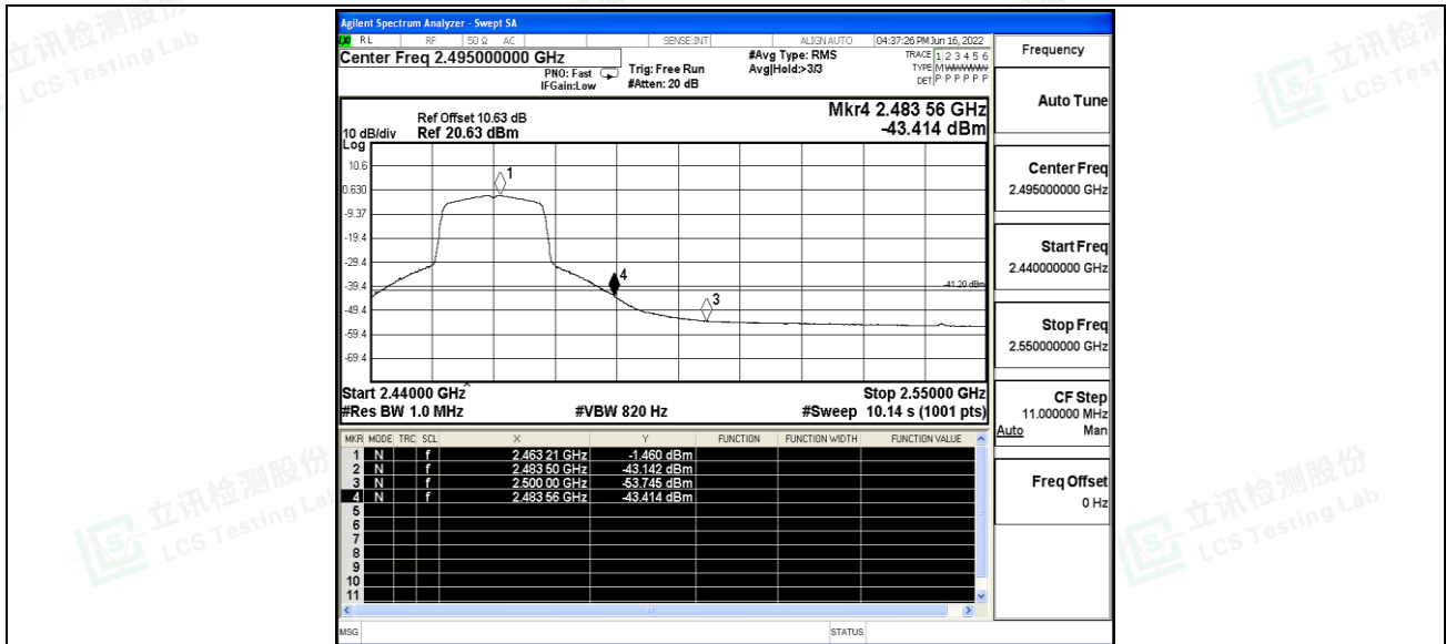
11N20SISO_Ant1_High_2462_Peak
