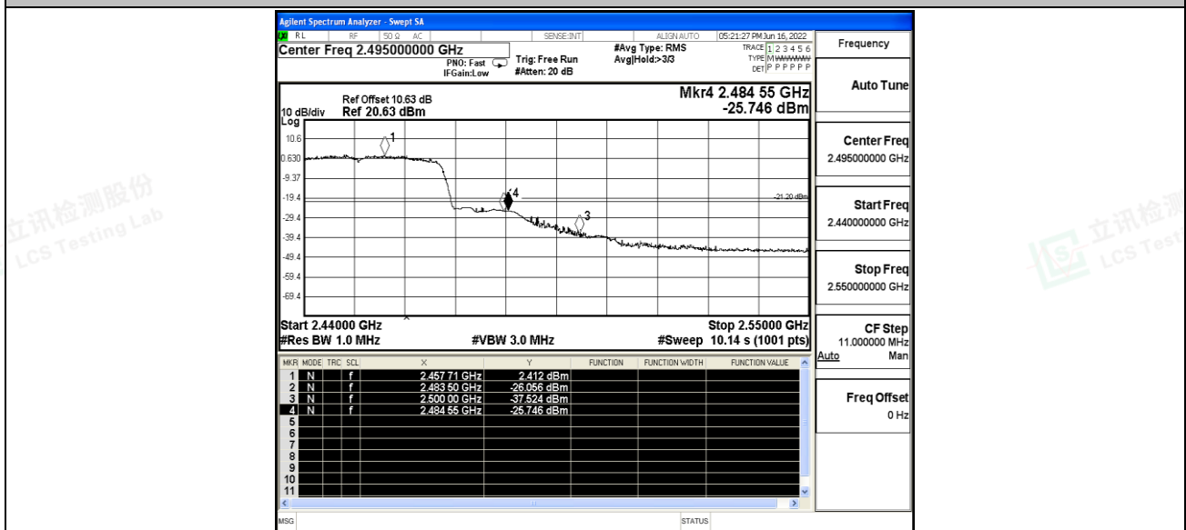
11N40SISO_Ant1_High_2452_Peak
