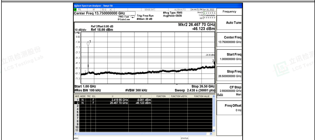
11N40SISO_Ant_2437_0~Reference
