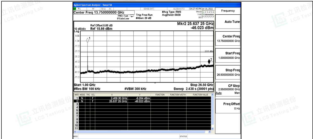
11N20SISO_Ant_2437_0~Reference
