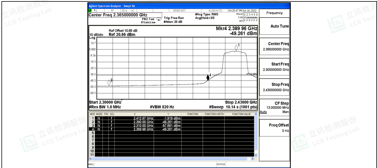
11N20SISO_Ant1_Low_2412_Peak
