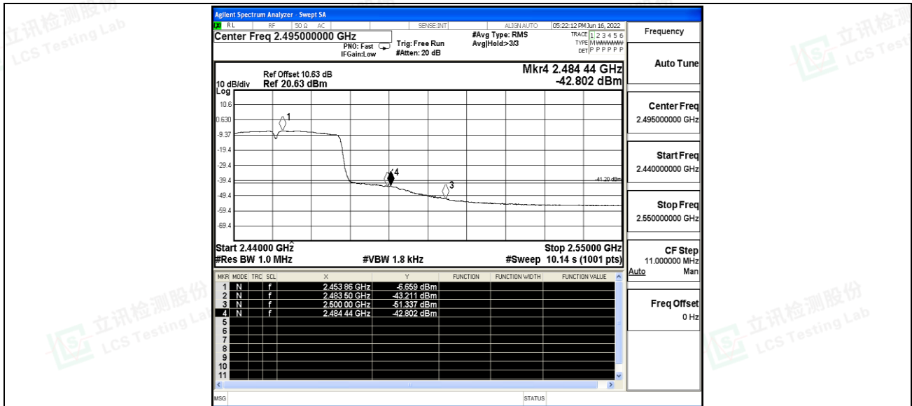
11N40SISO_Ant1_High_2452_Peak
