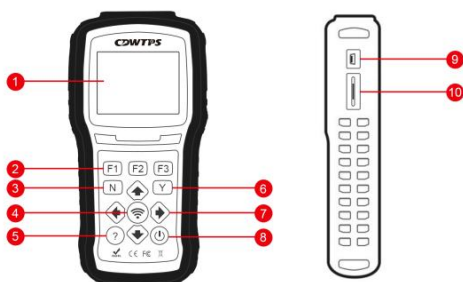
Figure 2-1 Front View
