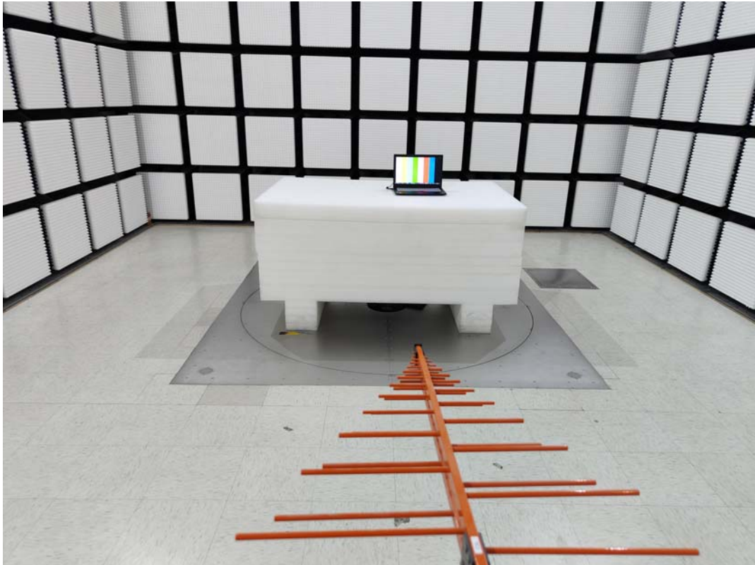
Radiated Emission Below 1GHz View-2
