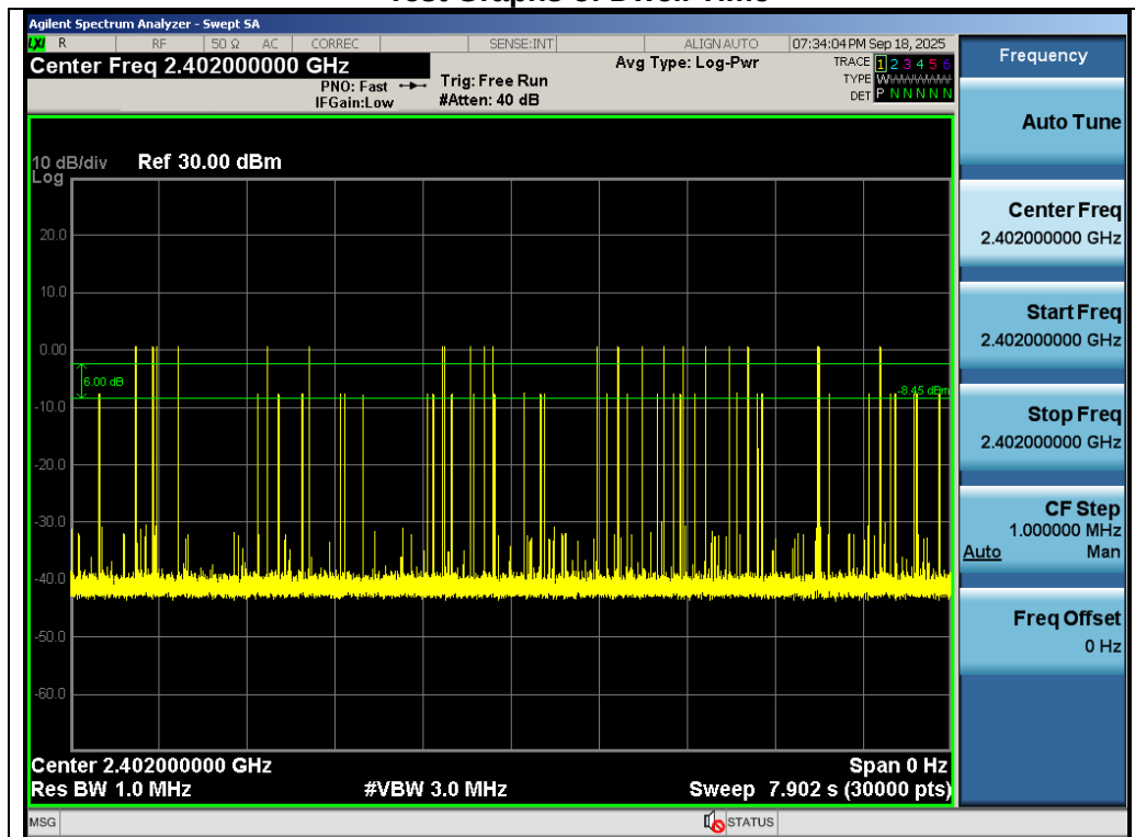
Test_Graph_2.4G_HOP_ANT1_NA_GFSK_2402_Number of Burst
