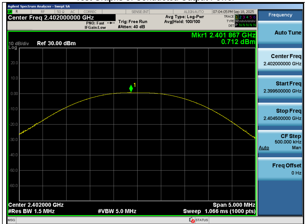
Test_Graph_2.4G_ANT1_2402_GFSK_Peak Power
