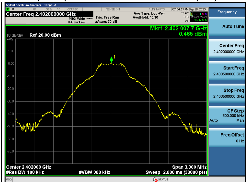
Test_Graph_2.4G_ANT1_2402_GFSK_Reference Level
