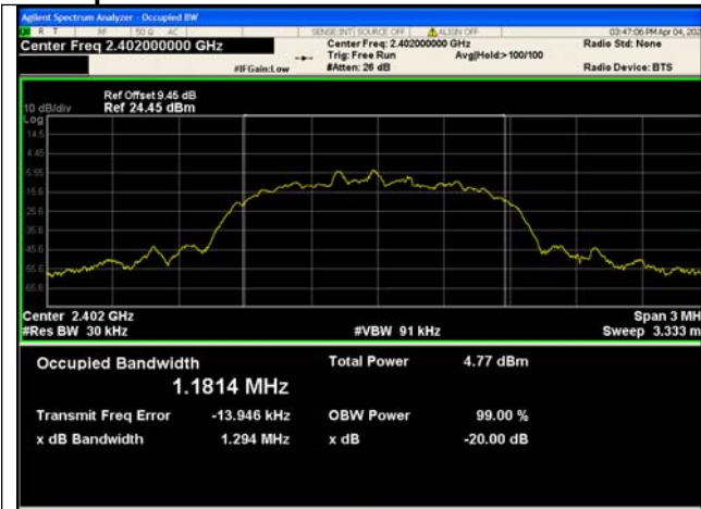
8DPSK_3-DH5_Channel 0
