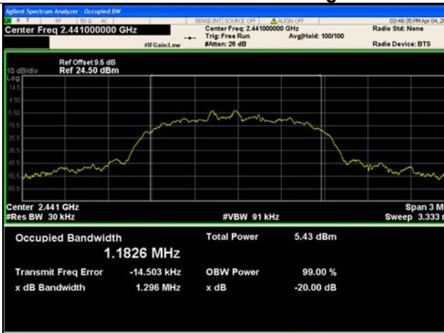
8DPSK_3-DH5_Channel 39
