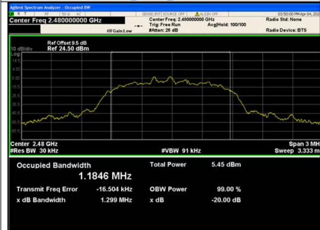
8DPSK_3-DH5_Channel 78
