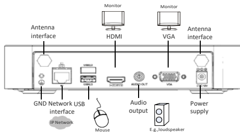
Figure 4-1 NVR Interfaces
