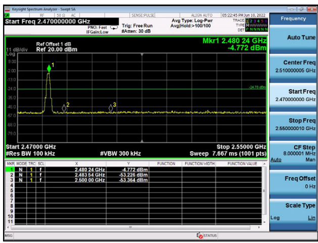
Right bandedge
