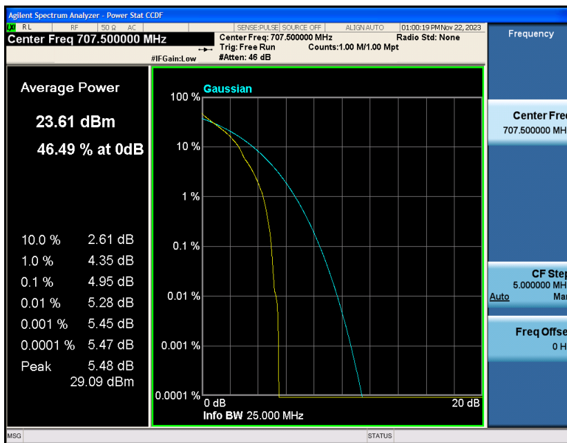
Band12-10MHz-QPSK-23095-50RB#0
