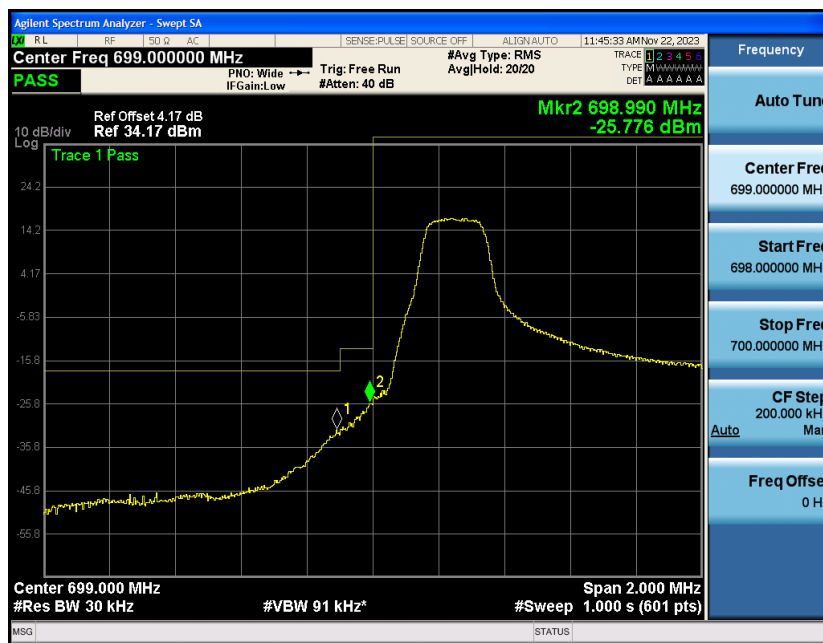
Band12-1.4MHz-QPSK-23017-1RB#5
