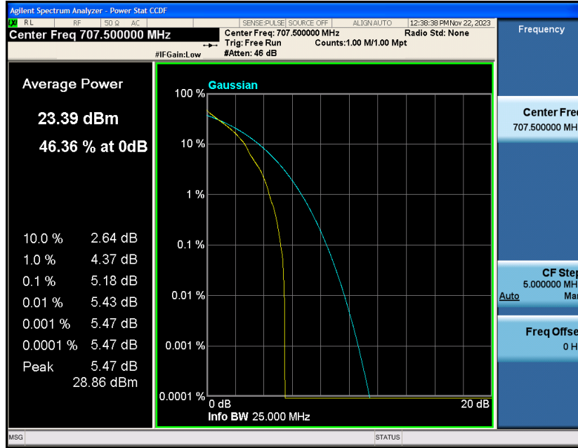
Band12-5MHz-QPSK-23095-25RB#0
