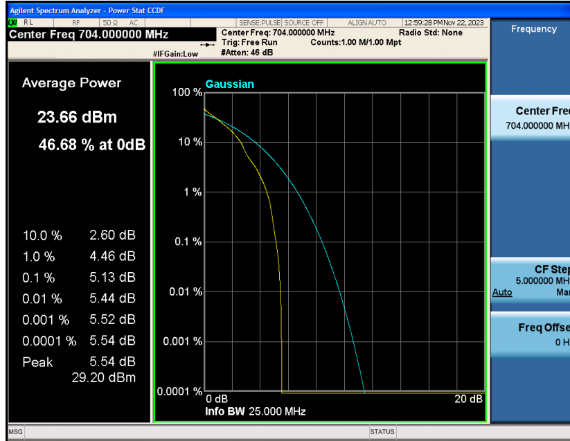
Band12-10MHz-QPSK-23060-50RB#0
