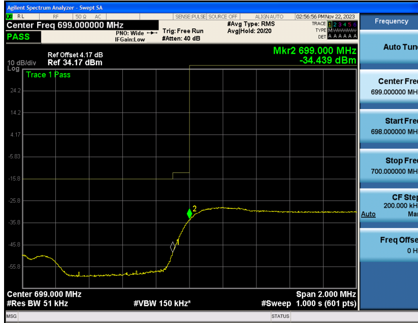
Band12-3MHz-QPSK-23025-15RB#0
