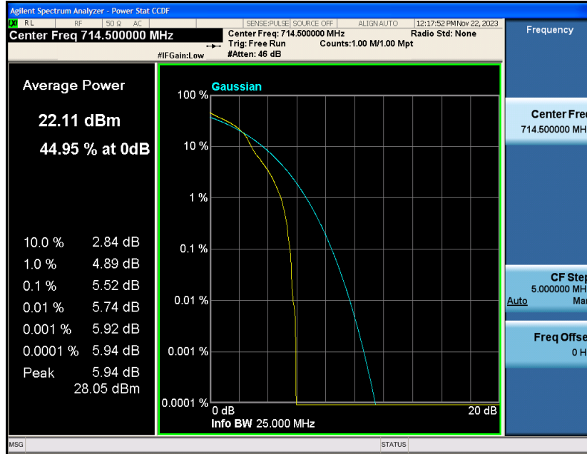
Band12-3MHz-16QAM-23165-15RB#0
