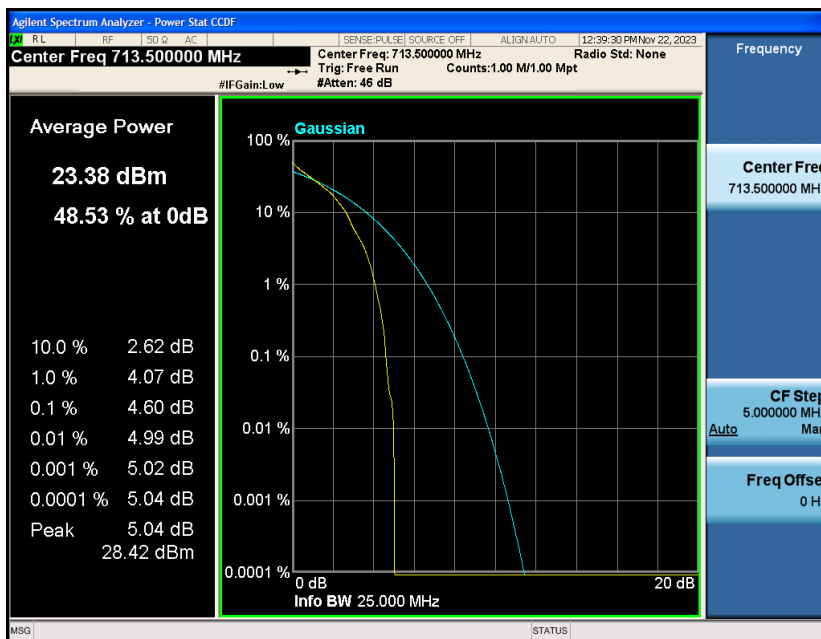
Band12-5MHz-QPSK-23155-25RB#0
