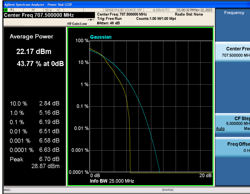
Band12-10MHz-16QAM-23095-50RB#0
