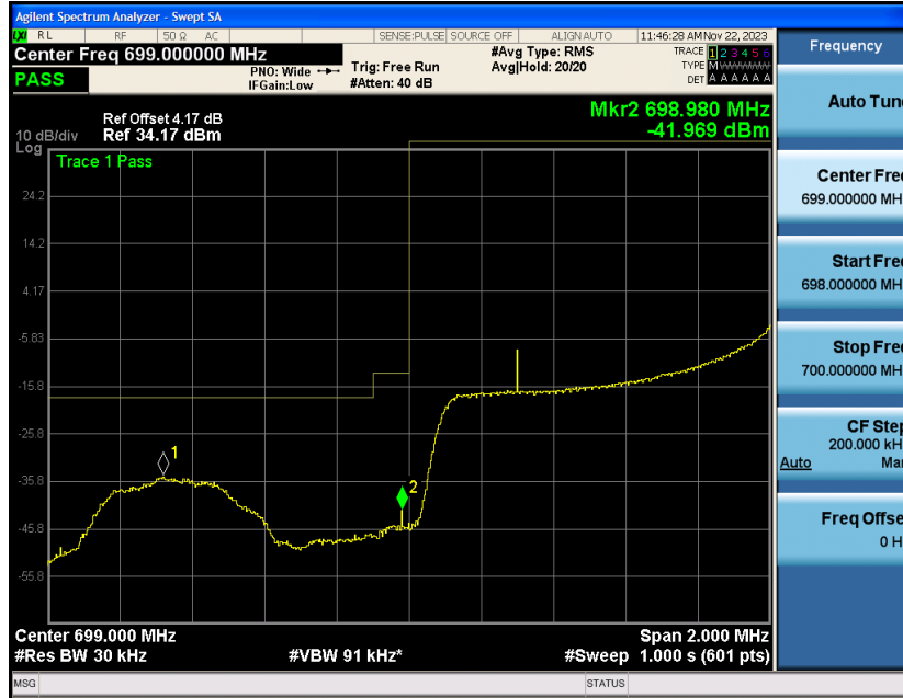
Band12-1.4MHz-QPSK-23017-6RB#0
