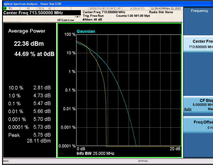
Band12-5MHz-16QAM-23155-25RB#0
