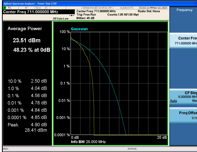
Band12-10MHz-QPSK-23130-50RB#0
