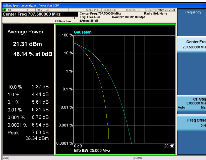
Band12-10MHz-QPSK-23130-1RB#0
