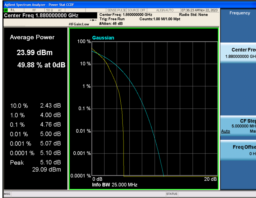
Band2-1.4MHz-QPSK-18900-6RB#0
