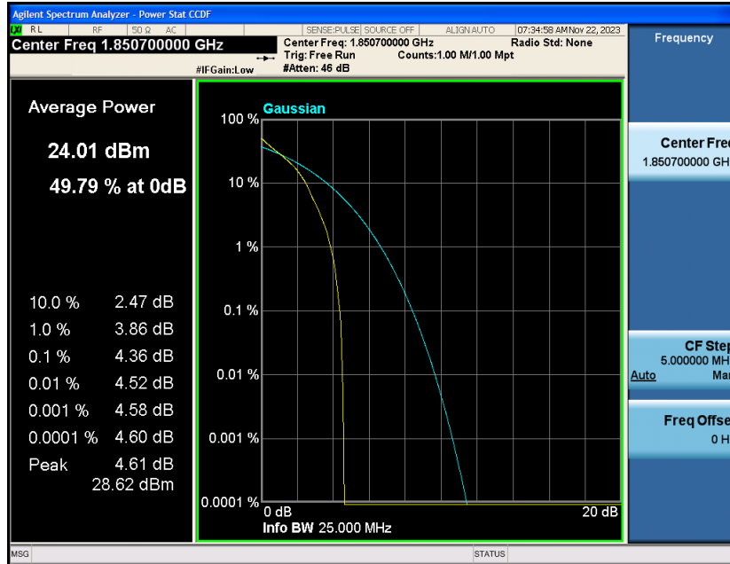
Band2-1.4MHz-QPSK-18607-6RB#0
