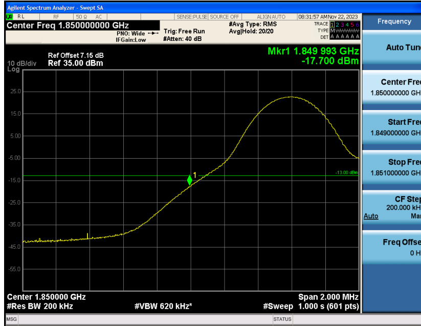
Band2-10MHz-16QAM-18650-1RB#49
