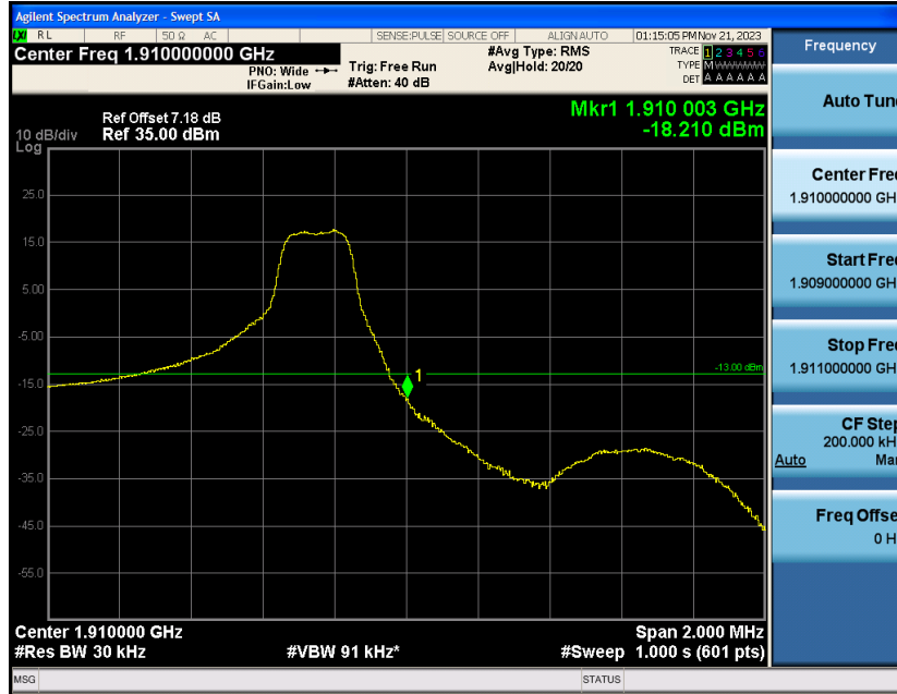
Band2-1.4MHz-16QAM-19193-6RB#0
