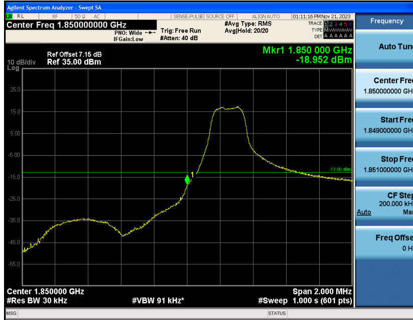
Band2-1.4MHz-16QAM-18607-1RB#5
