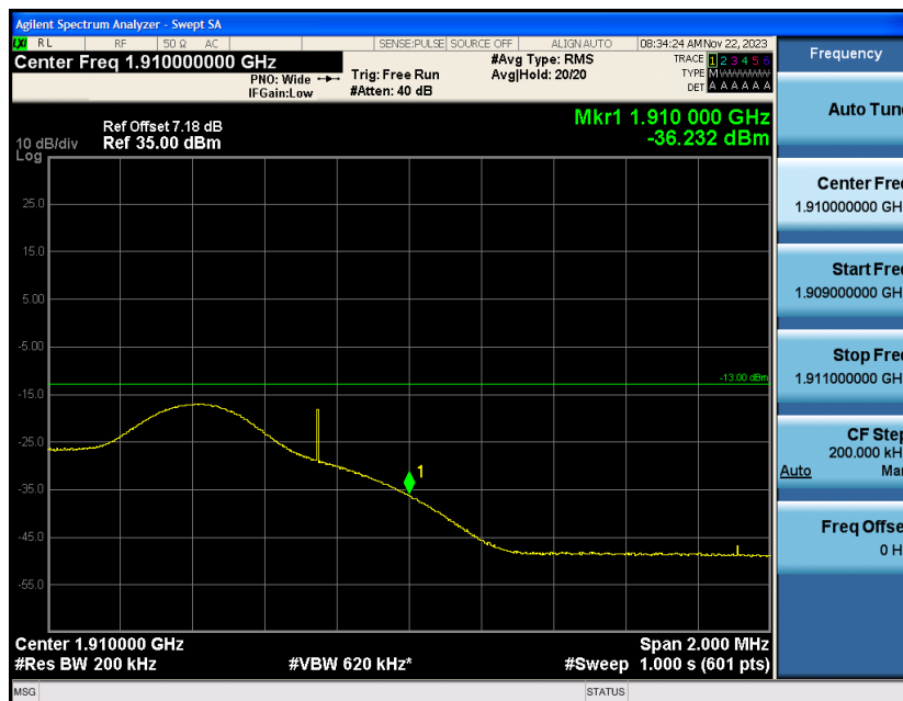
Band2-10MHz-QPSK-19150-1RB#49
