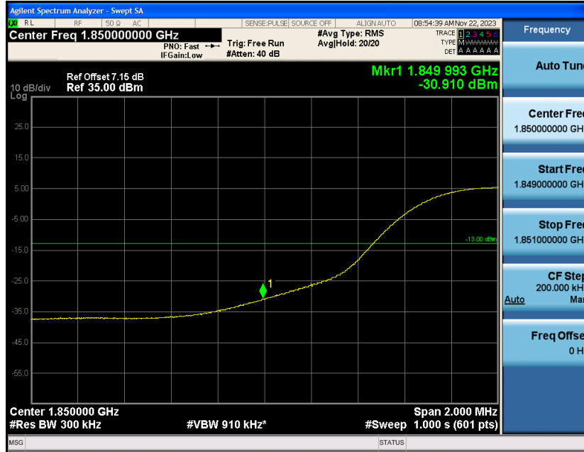
Band2-15MHz-QPSK-19125-1RB#0
