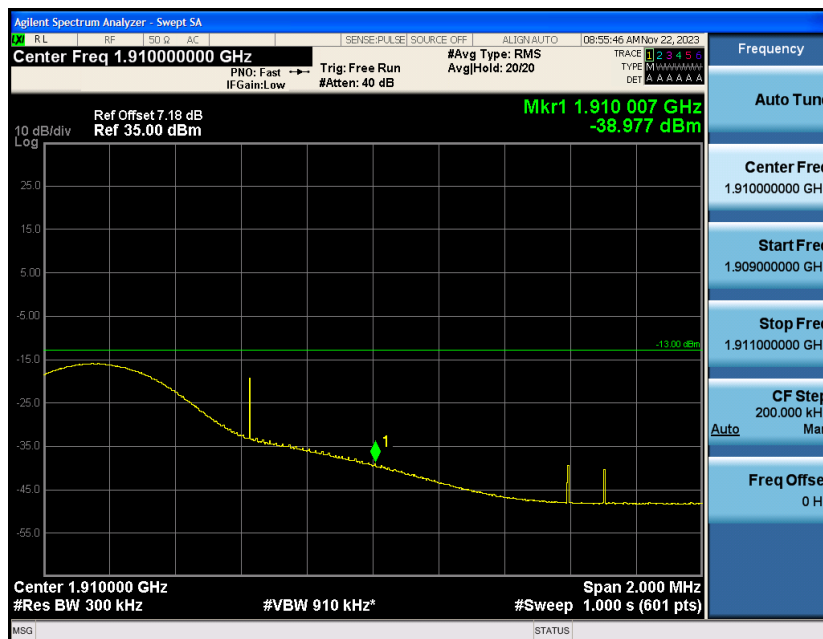
Band2-15MHz-QPSK-19125-1RB#74
