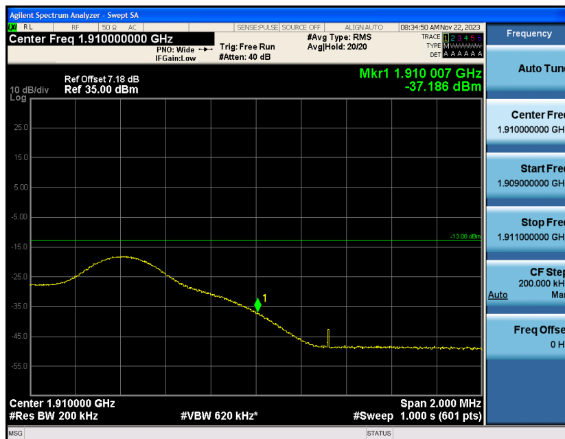
Band2-10MHz-16QAM-19150-1RB#49
