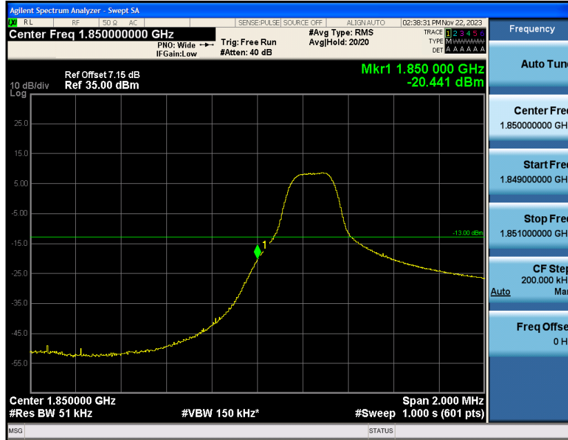
Band2-3MHz-16QAM-18615-1RB#14
