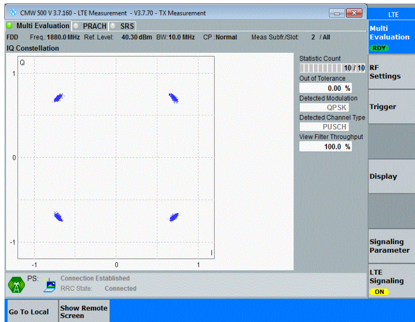
Band2-10MHz-QPSK-19150-50RB#0
