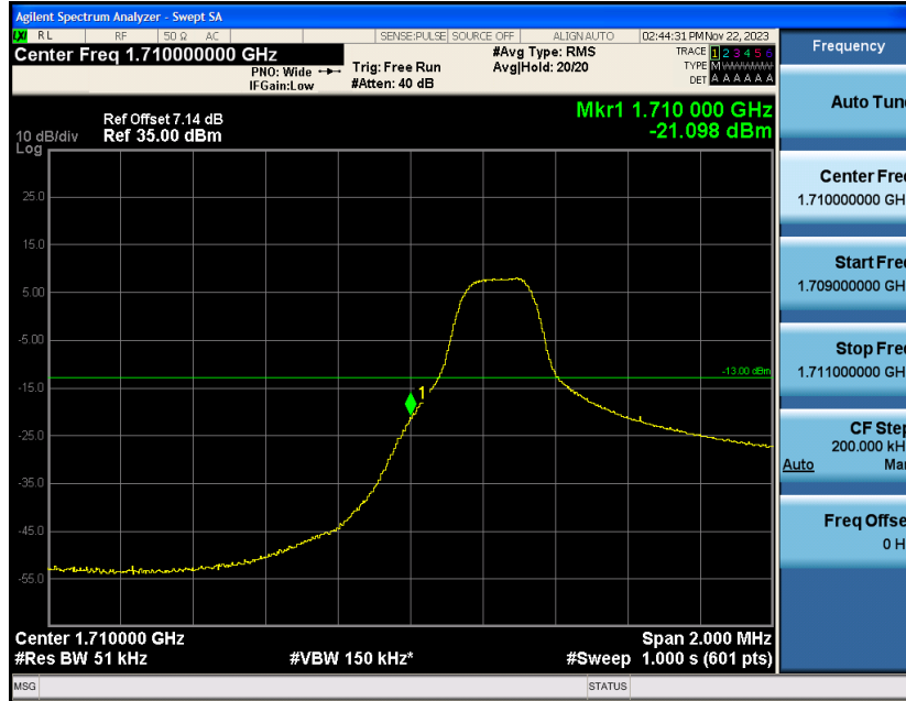
Band4-3MHz-16QAM-19965-1RB#14
