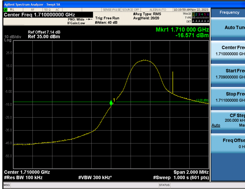
Band4-5MHz-16QAM-19975-1RB#24
