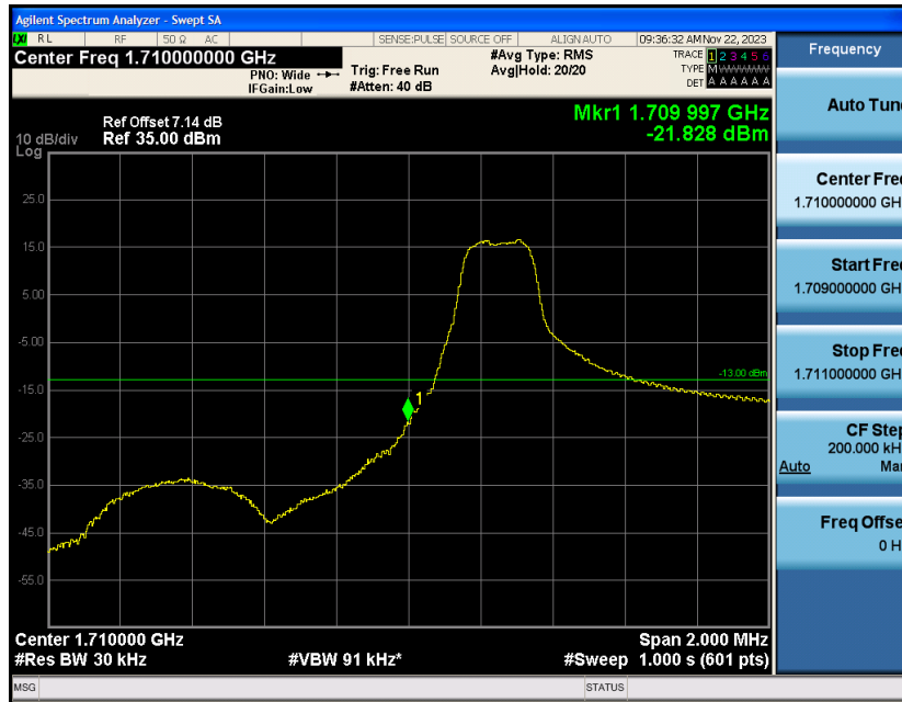
Band4-1.4MHz-16QAM-19957-1RB#5
