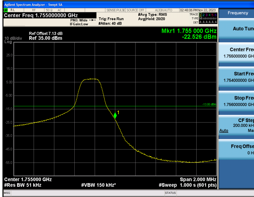
Band4-3MHz-16QAM-20385-15RB#0
