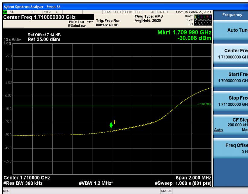
Band4-20MHz-16QAM-20300-1RB#0
