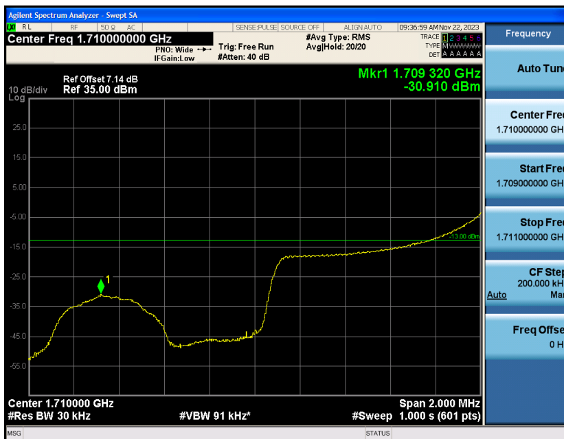
Band4-1.4MHz-QPSK-19957-6RB#0
