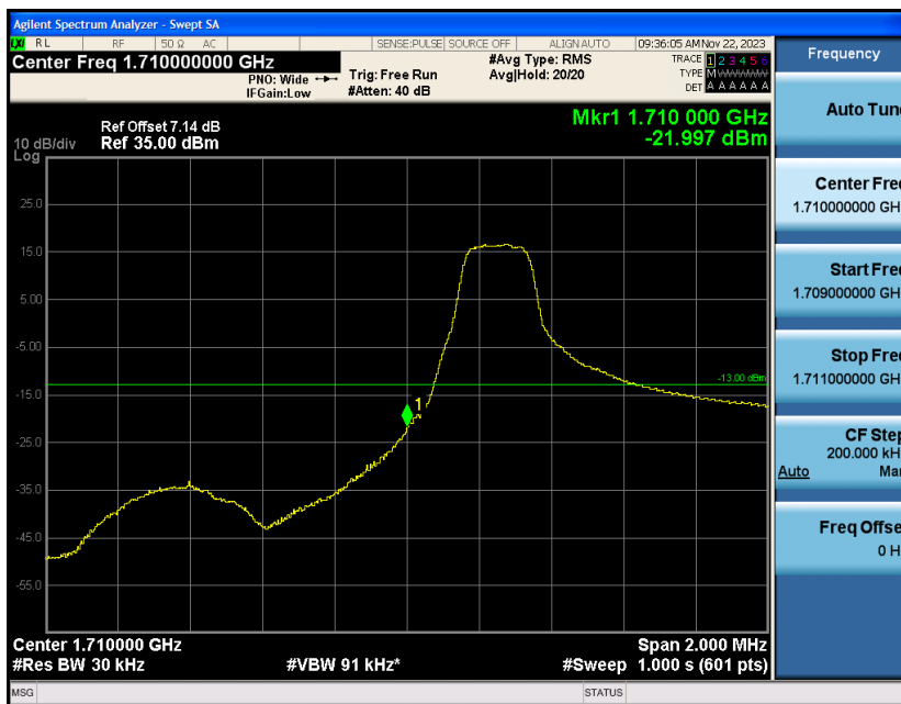
Band4-1.4MHz-QPSK-19957-1RB#5
