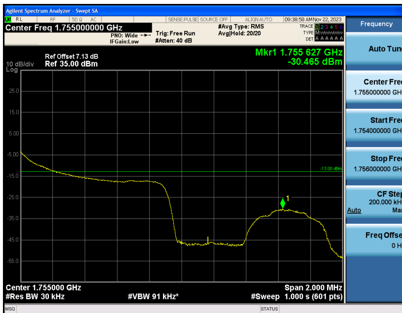
Band4-1.4MHz-QPSK-20393-1RB#5
