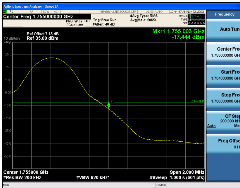
Band4-10MHz-QPSK-20350-50RB#0
