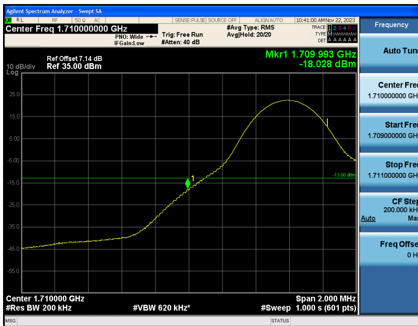
Band4-10MHz-QPSK-20000-1RB#49
