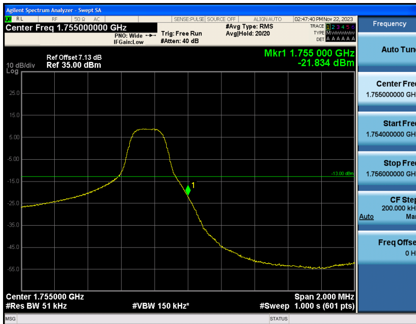
Band4-3MHz-QPSK-20385-15RB#0
