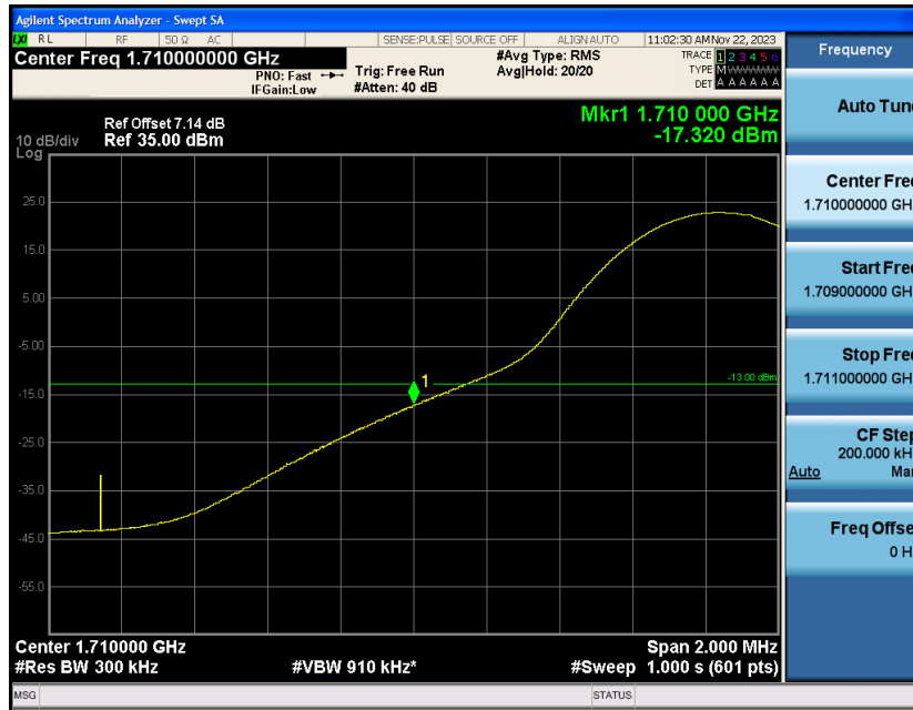
Band4-15MHz-QPSK-20025-1RB#74
