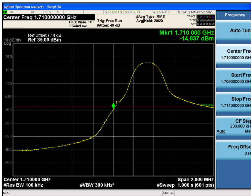
Band4-5MHz-QPSK-19975-1RB#24
