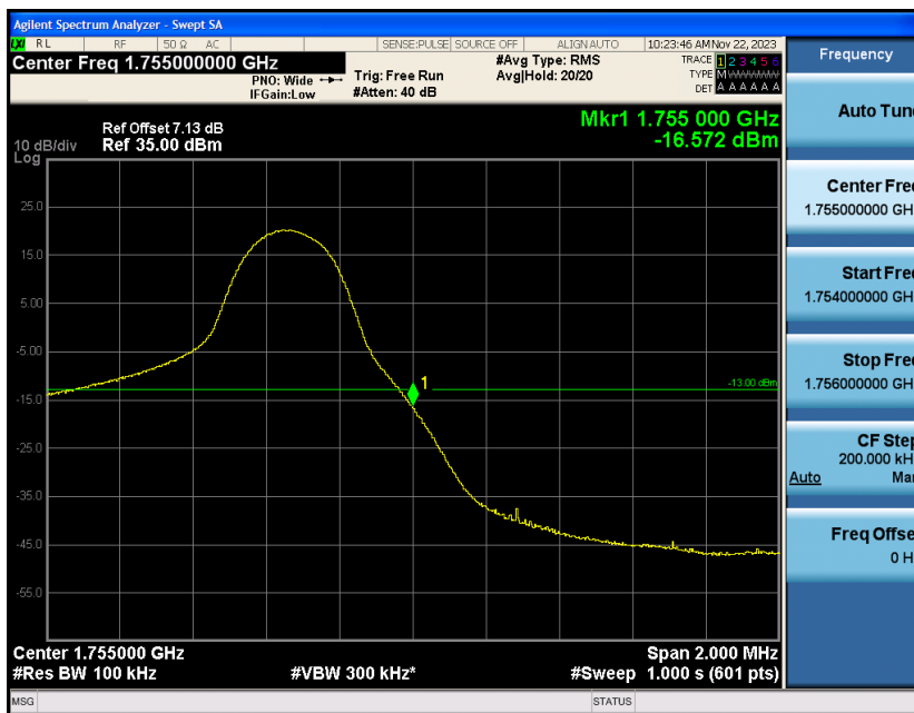
Band4-5MHz-16QAM-20375-25RB#0
