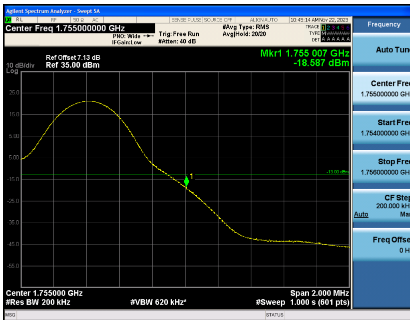
Band4-10MHz-16QAM-20350-50RB#0
