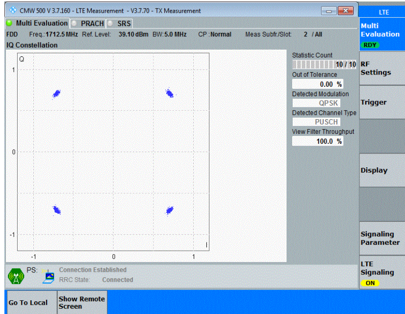
Band4-5MHz-QPSK-20175-25RB#0
