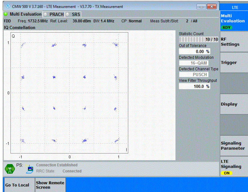
Band4-1.4MHz-16QAM-20393-6RB#0
