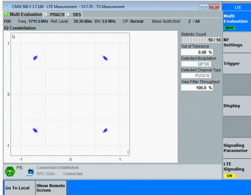
Band4-3MHz-QPSK-20175-15RB#0
