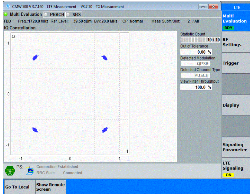
Band4-20MHz-QPSK-20175-100RB#0
