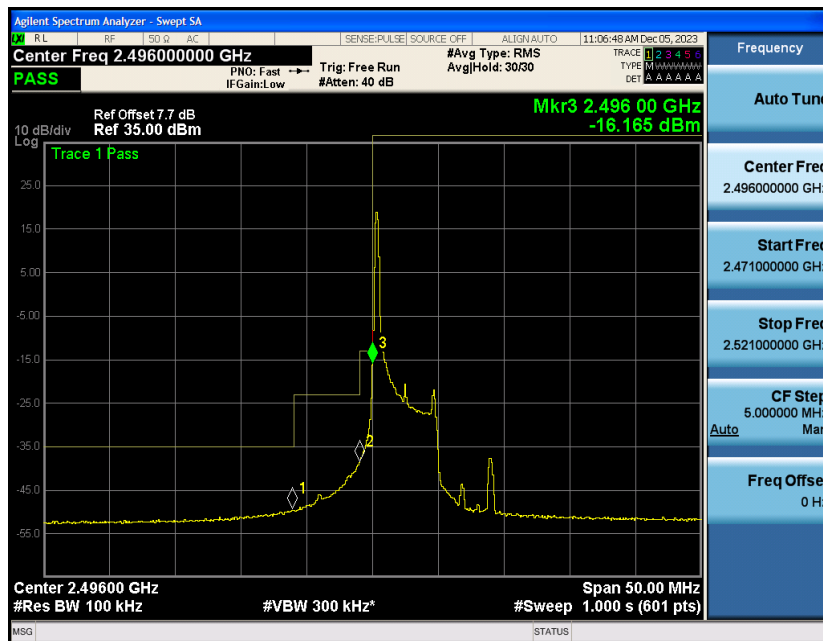
Band41-5MHz-16QAM-39675-1RB#24
