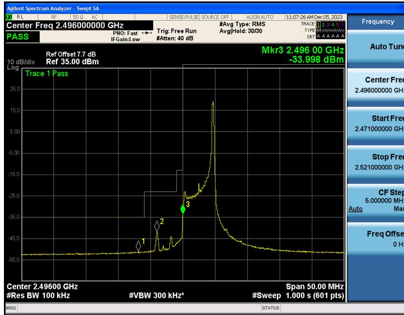
Band41-5MHz-QPSK-39675-25RB#0
