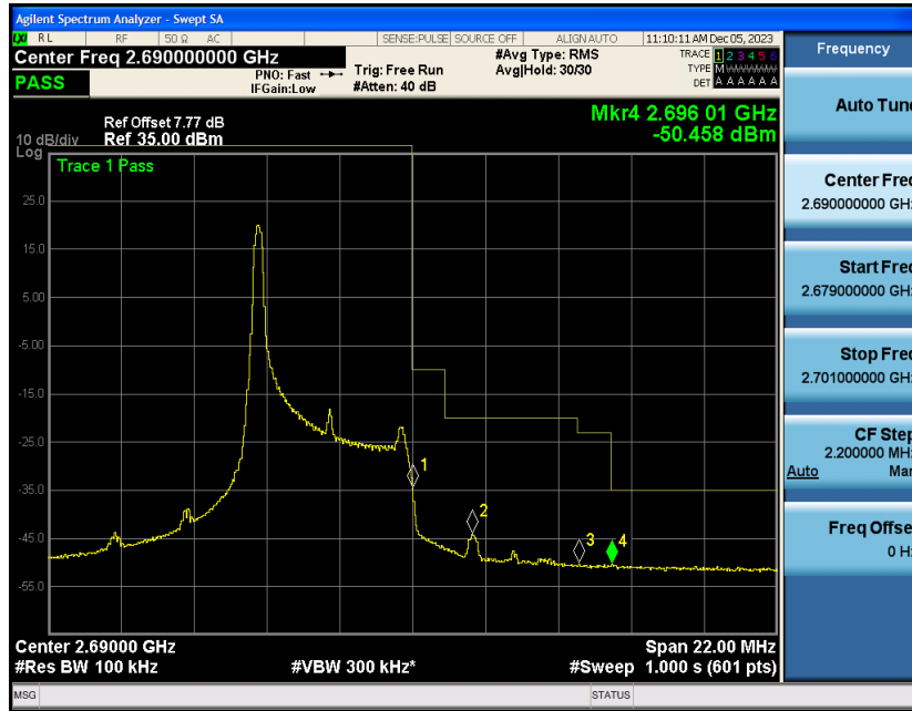
Band41-5MHz-QPSK-41565-1RB#24
