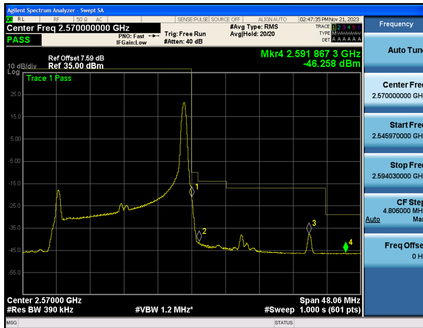
Band7-20MHz-16QAM-21350-100RB#0
