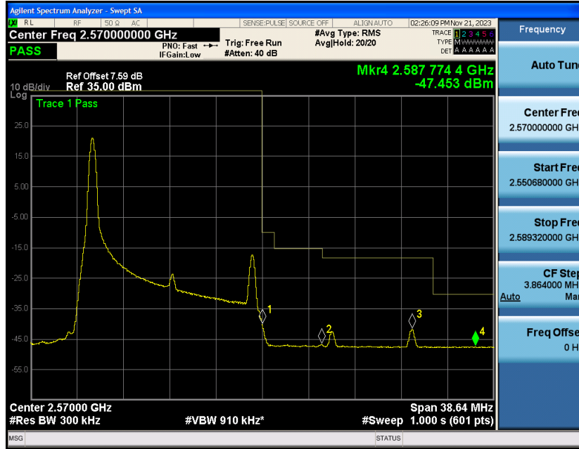
Band7-15MHz-16QAM-21375-1RB#74
