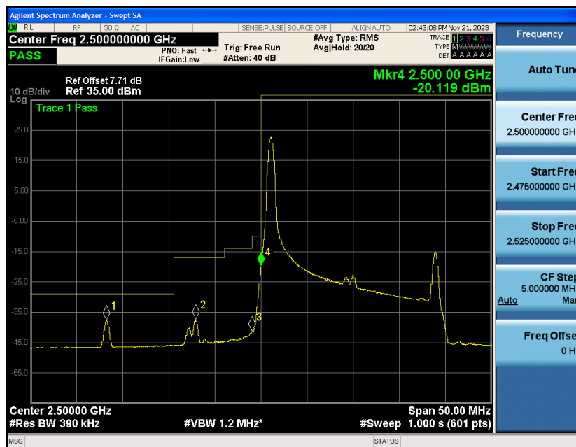
Band7-20MHz-QPSK-20850-1RB#99
