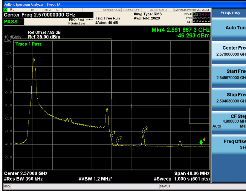
Band7-20MHz-16QAM-21350-1RB#99
