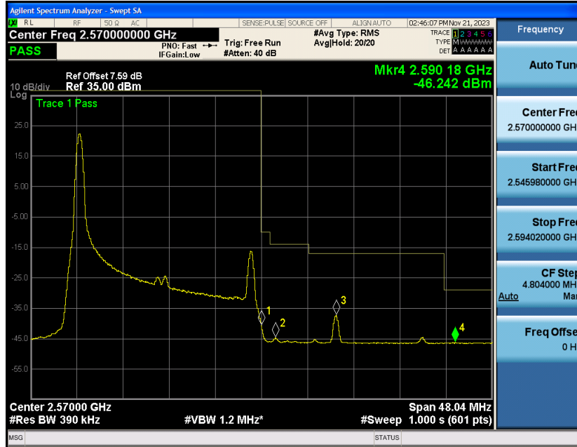
Band7-20MHz-QPSK-21350-1RB#99
