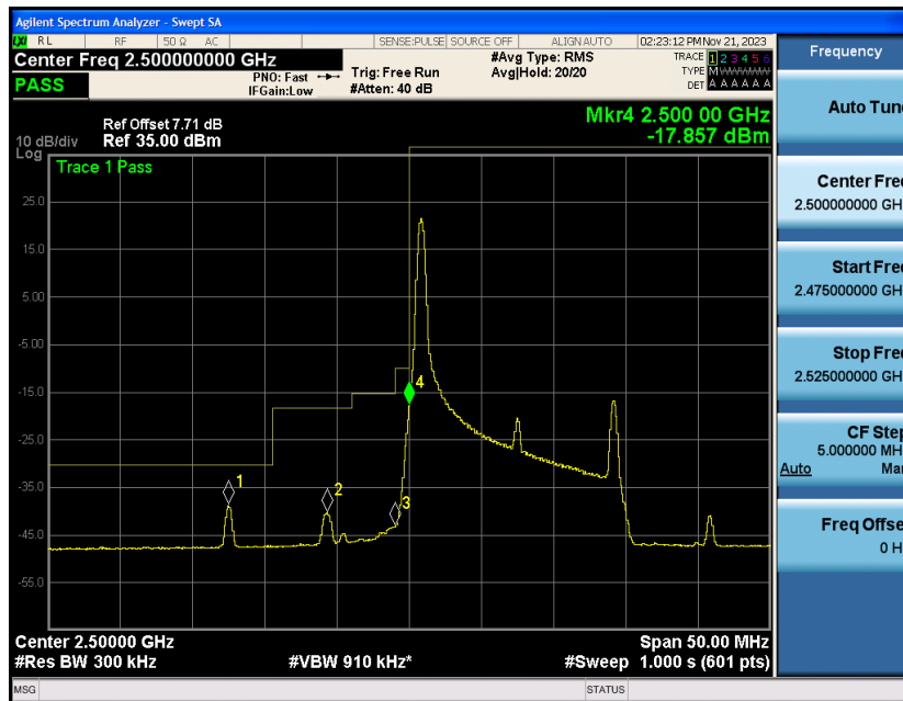
Band7-15MHz-16QAM-20825-1RB#74
