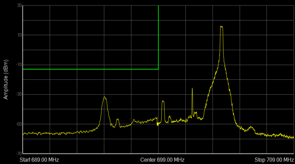
Band12 QAM16 BW=5MHz Channel=23035 RB Size=1 Position=#Max
