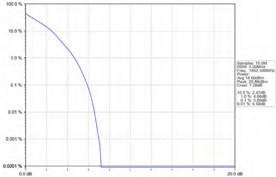
Band2_5MHz_QPSK_LCH_1852.5MHz_RB_25_0_NTNV
