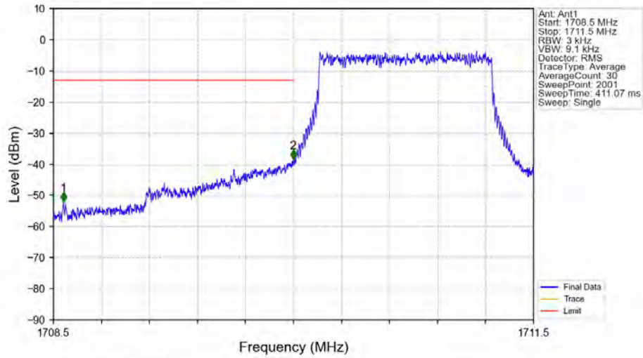
Band4_1.4MHz_QPSK_LCH_1710.7MHz_RB_1_0_NTNV
