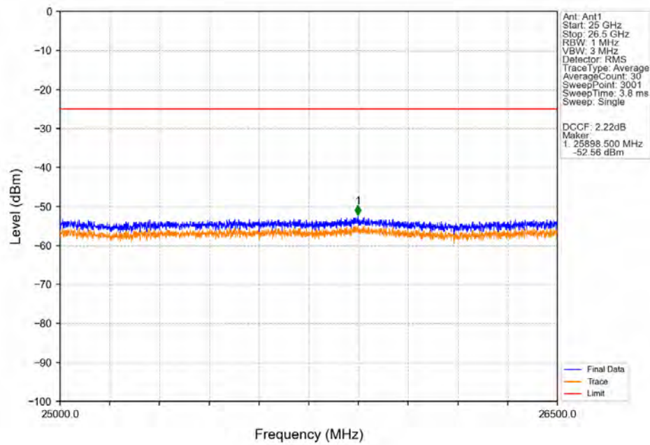
Band41_5MHz_16QAM_LCH_2557.5MHz_RB_25_0_NTNV
