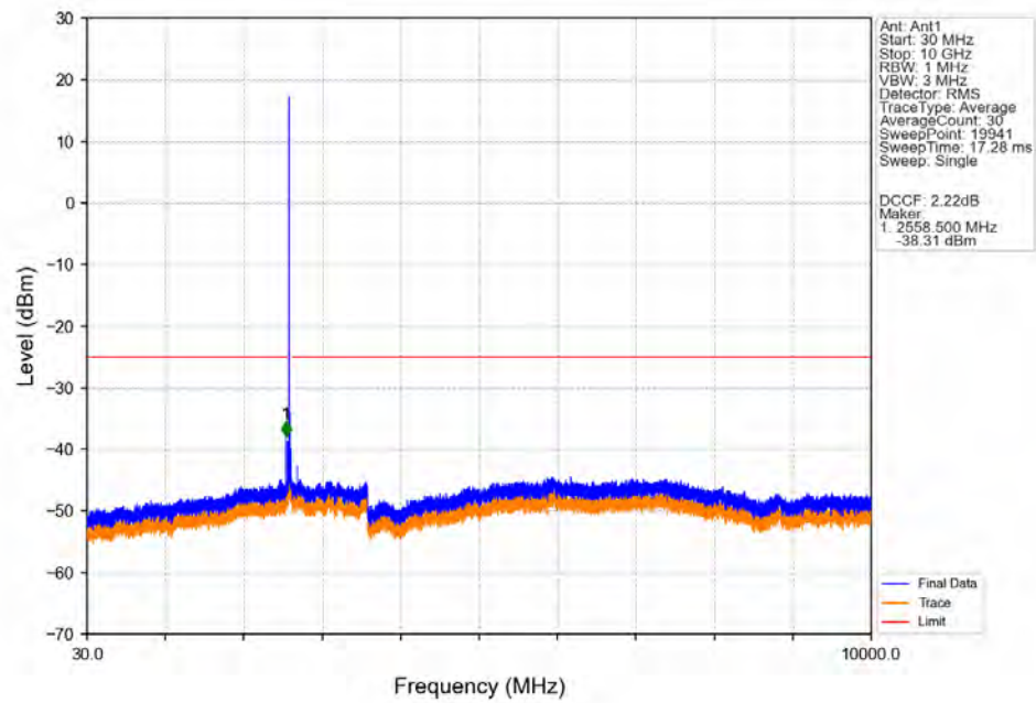
Band41_15MHz_16QAM_MCH_2605MHz_RB_1_0_NTNV
