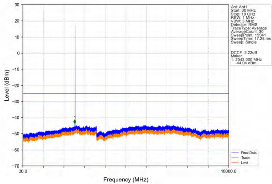
Band41_5MHz_16QAM_LCH_2557.5MHz_RB_1_0_NTNV
