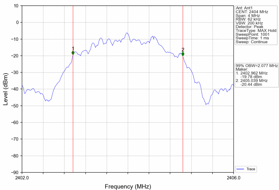
2M_LCH_2404MHz_Ant1_NTNV
