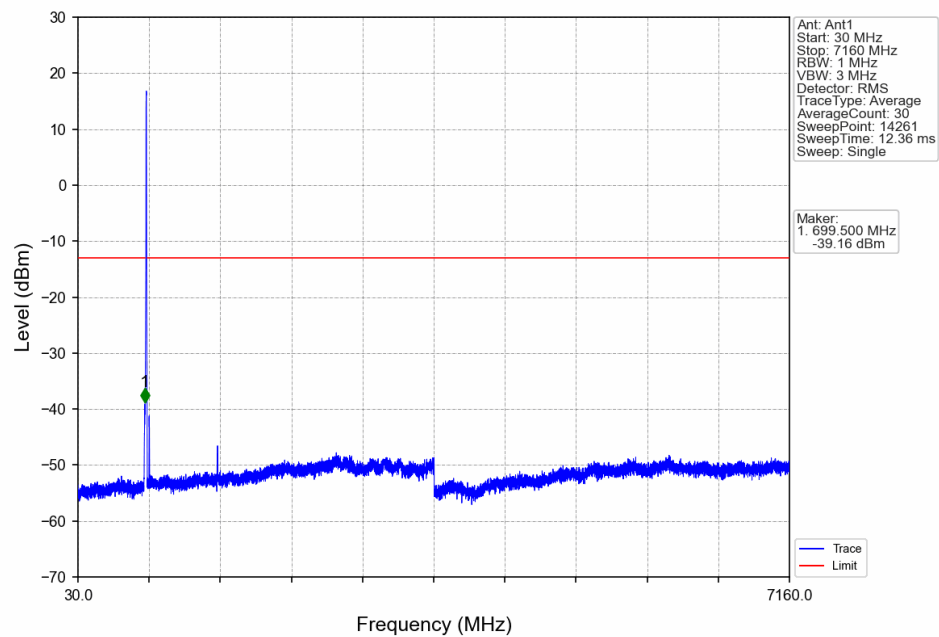
Band17_5MHz_QPSK_HCH_713.5MHz_RB_1_24_NTNV
