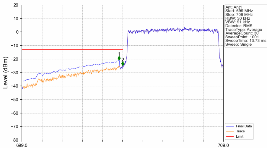
Band17_5MHz_16QAM_LCH_706.5MHz_RB_25_0_NTNV
