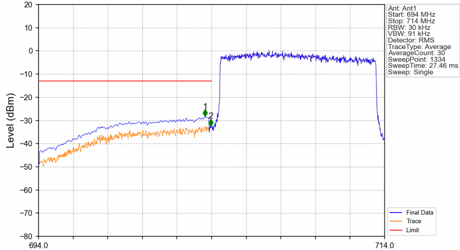
Band17_10MHz_16QAM_LCH_709MHz_RB_50_0_NTNV
