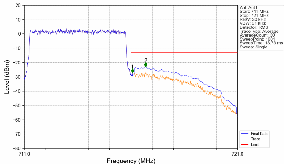
Band17_5MHz_QPSK_HCH_713.5MHz_RB_1_24_NTNV
