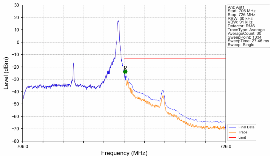
Band17_10MHz_QPSK_HCH_711MHz_RB_1_49_NTNV
