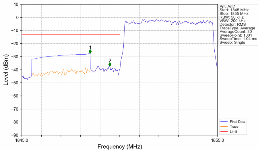
Band2_5MHz_QPSK_LCH_1852.5MHz_RB_25_0_NTNV
