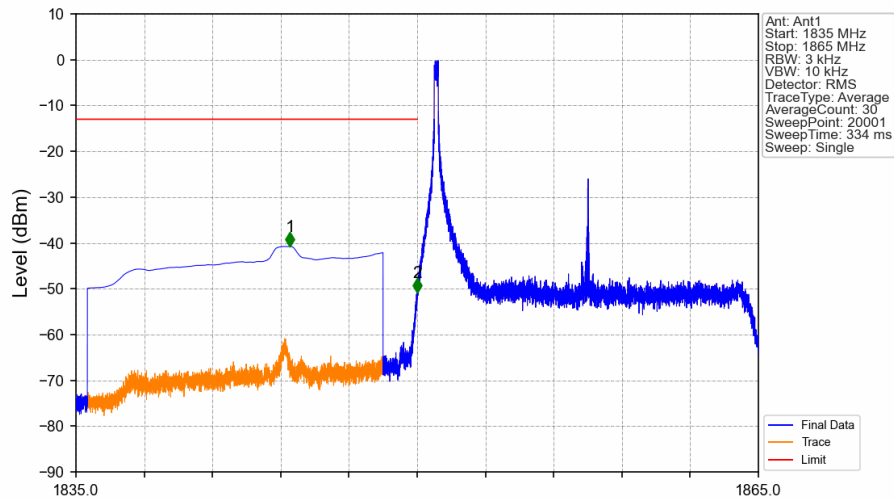
Band2_15MHz_16QAM_LCH_1857.5MHz_RB_1_0_NTNV
