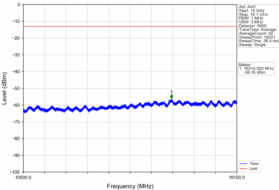
Band2_15MHz_QPSK_LCH_1857.5MHz_RB_75_0_NTNV
