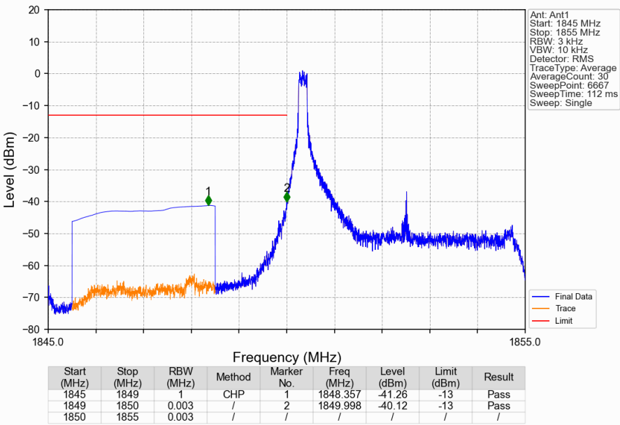
Band2_5MHz_16QAM_LCH_1852.5MHz_RB_1_0_NTNV
