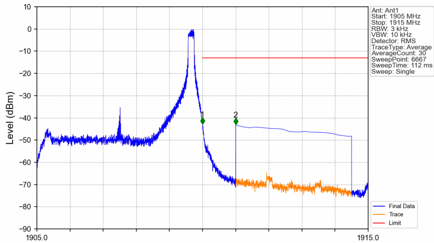
Band2_5MHz_16QAM_HCH_1907.5MHz_RB_1_24_NTNV
