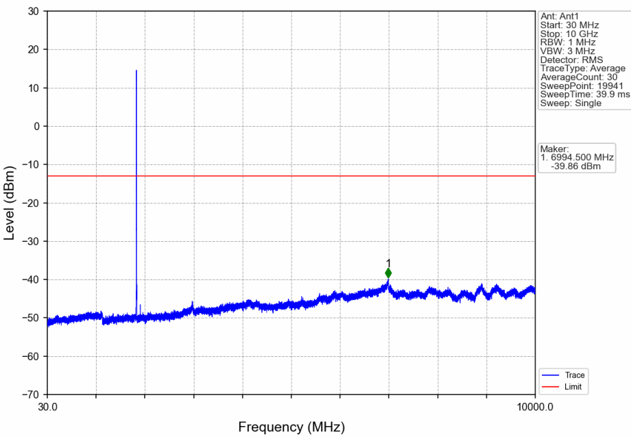
Band2_5MHz_16QAM_LCH_1852.5MHz_RB_1_0_NTNV
