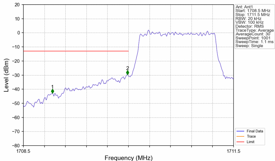
Band4_1.4MHz_QPSK_LCH_1710.7MHz_RB_6_0_NTNV
