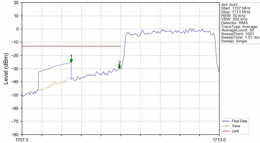
Band4_3MHz_16QAM_LCH_1711.5MHz_RB_15_0_NTNV
