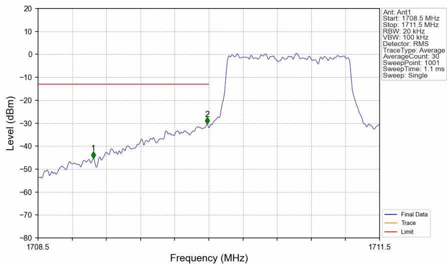
Band4_1.4MHz_16QAM_LCH_1710.7MHz_RB_6_0_NTNV
