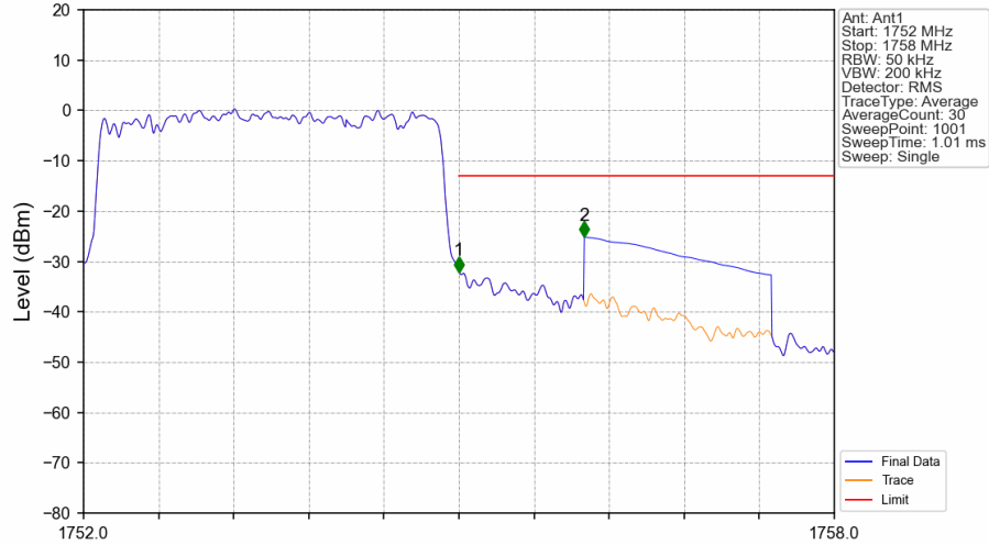
Band4_3MHz_16QAM_HCH_1753.5MHz_RB_15_0_NTNV
