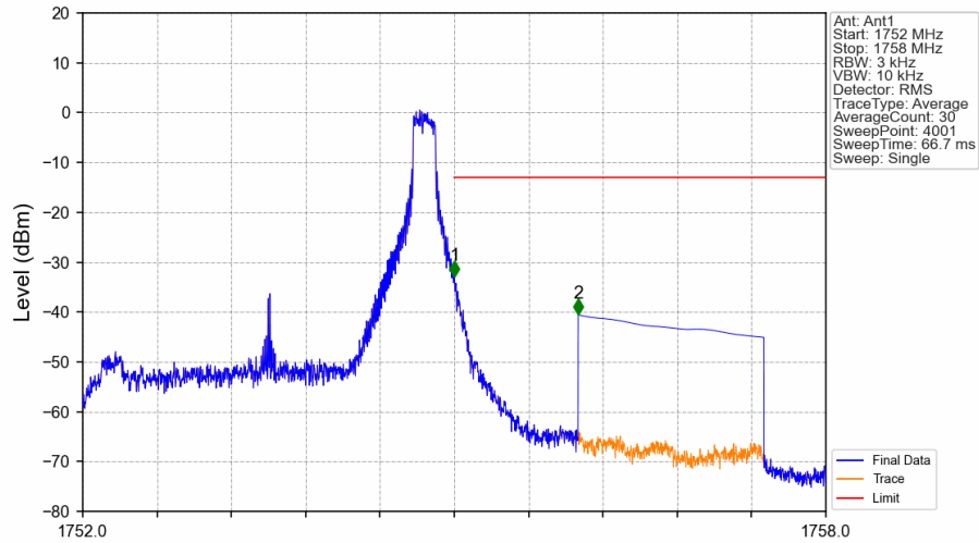
Band4_3MHz_16QAM_HCH_1753.5MHz_RB_1_14_NTNV
