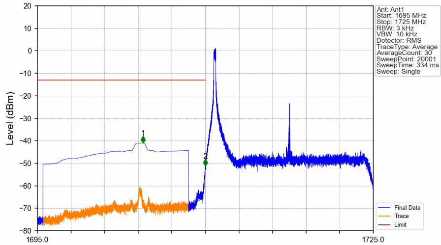
Band4_15MHz_16QAM_LCH_1717.5MHz_RB_1_0_NTNV
