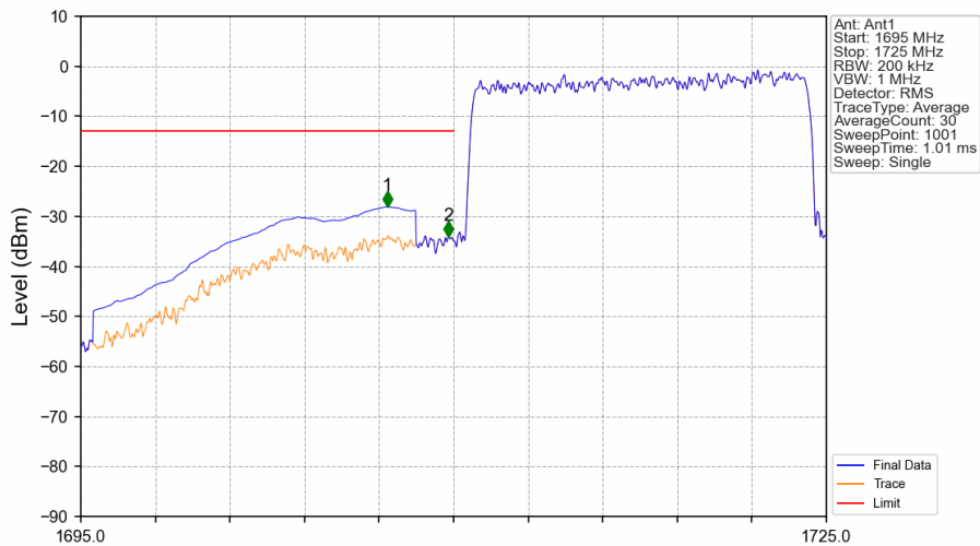
Band4_15MHz_16QAM_LCH_1717.5MHz_RB_75_0_NTNV
