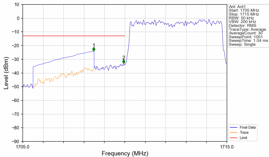
Band4_5MHz_QPSK_LCH_1712.5MHz_RB_25_0_NTNV
