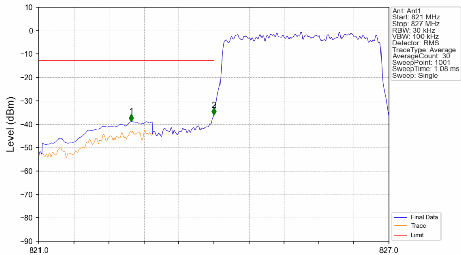
Band5_3MHz_QPSK_LCH_825.5MHz_RB_15_0_NTNV
