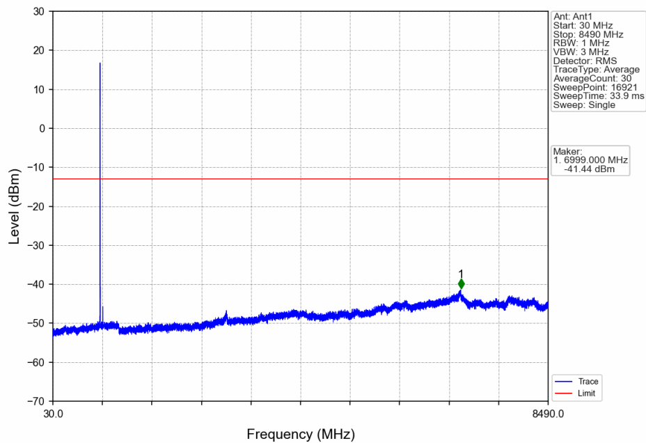
Band5_3MHz_QPSK_MCH_836.5MHz_RB_1_0_NTNV
