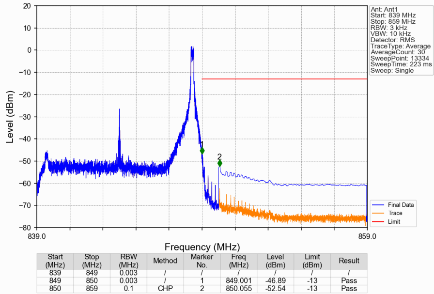
Band5_10MHz_16QAM_HCH_844MHz_RB_1_49_NTNV
