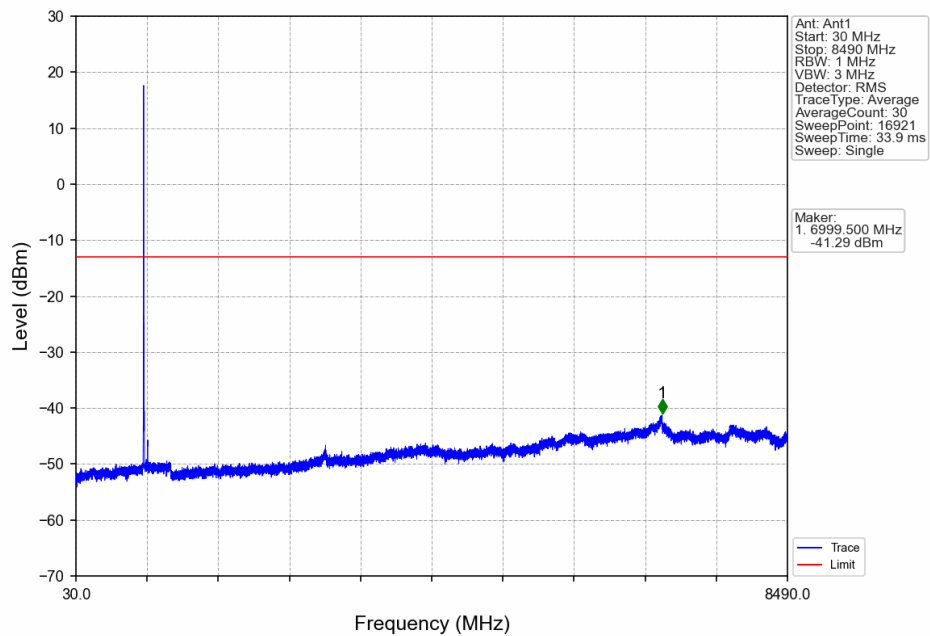
Band5_5MHz_QPSK_MCH_836.5MHz_RB_1_0_NTNV
