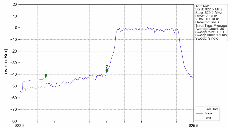
Band5_1.4MHz_16QAM_LCH_824.7MHz_RB_6_0_NTNV
