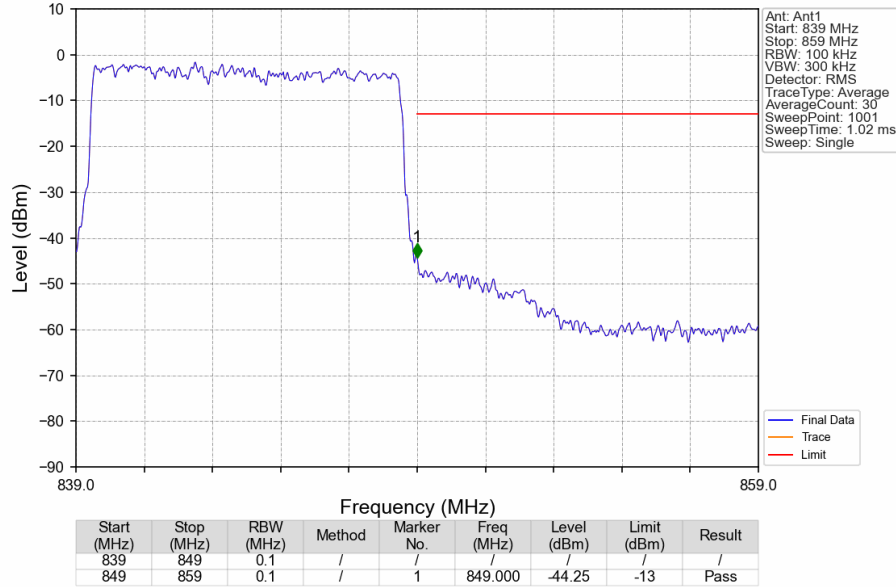
Band5_10MHz_16QAM_HCH_844MHz_RB_50_0_NTNV
