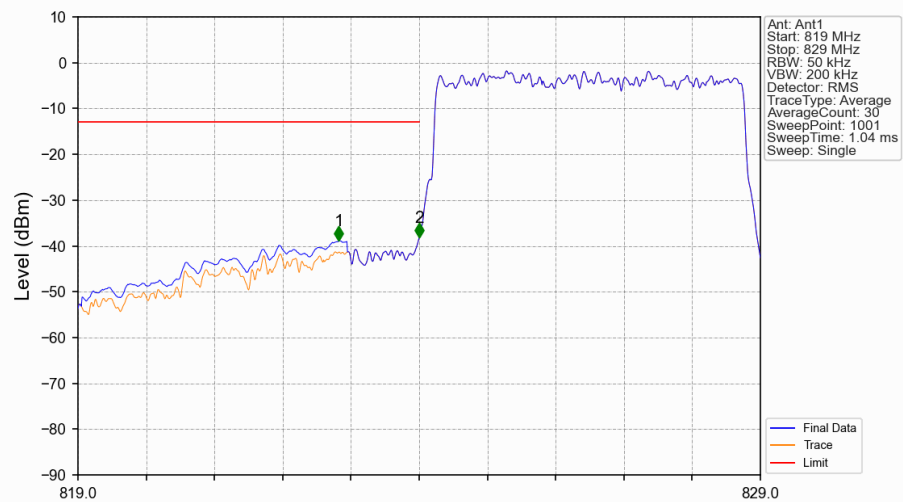
Band5_5MHz_16QAM_LCH_826.5MHz_RB_25_0_NTNV
