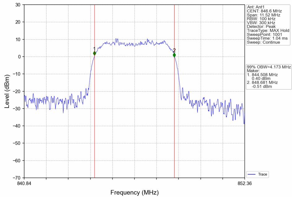
Band5_HSUPA_HCH_846.6MHz_Subtest 1_NTNV
