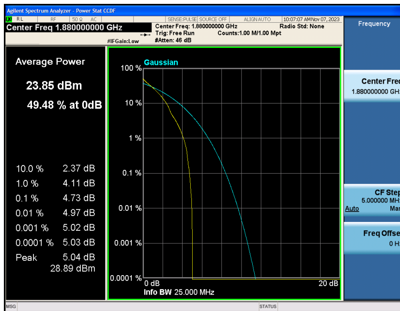
Band2-3MHz-QPSK-18900-15RB#0
