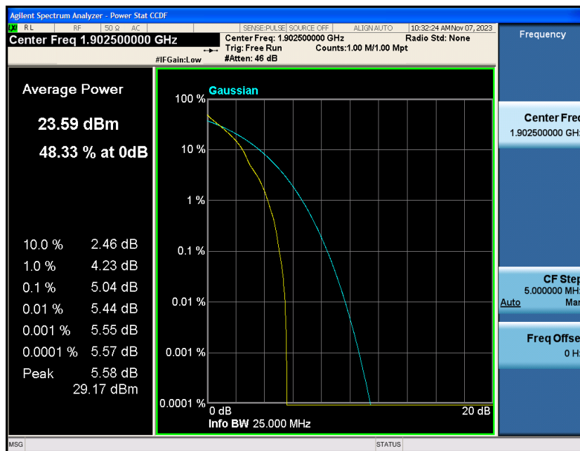
Band2-15MHz-QPSK-19125-75RB#0
