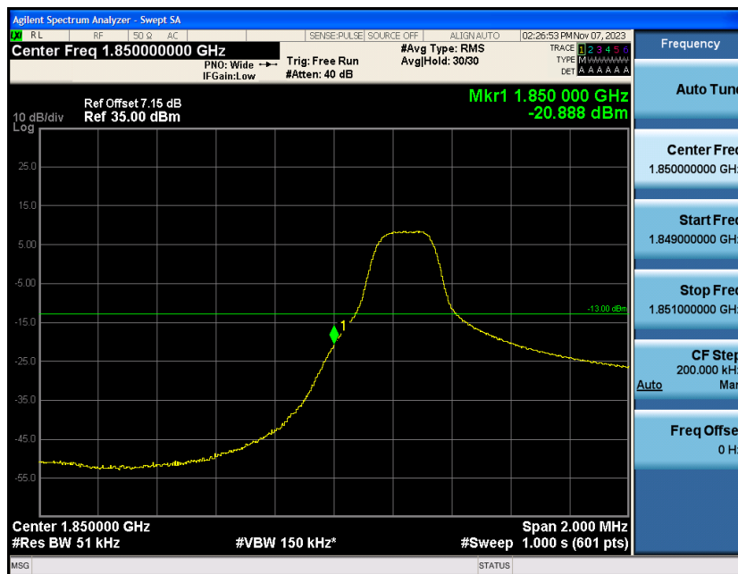
Band2-3MHz-16QAM-18615-1RB#14
