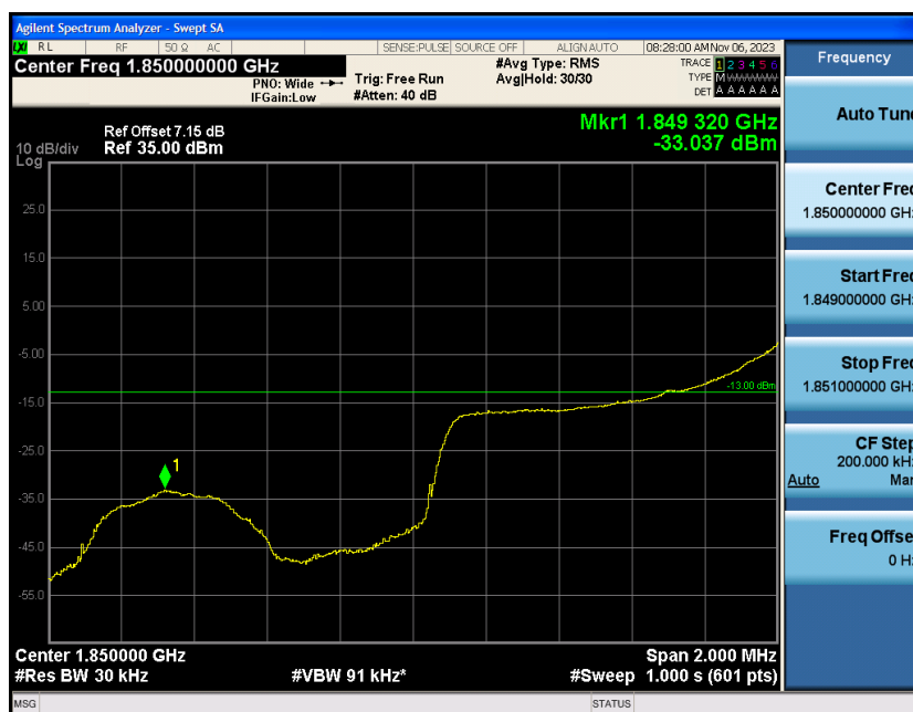
Band2-1.4MHz-QPSK-18607-6RB#0
