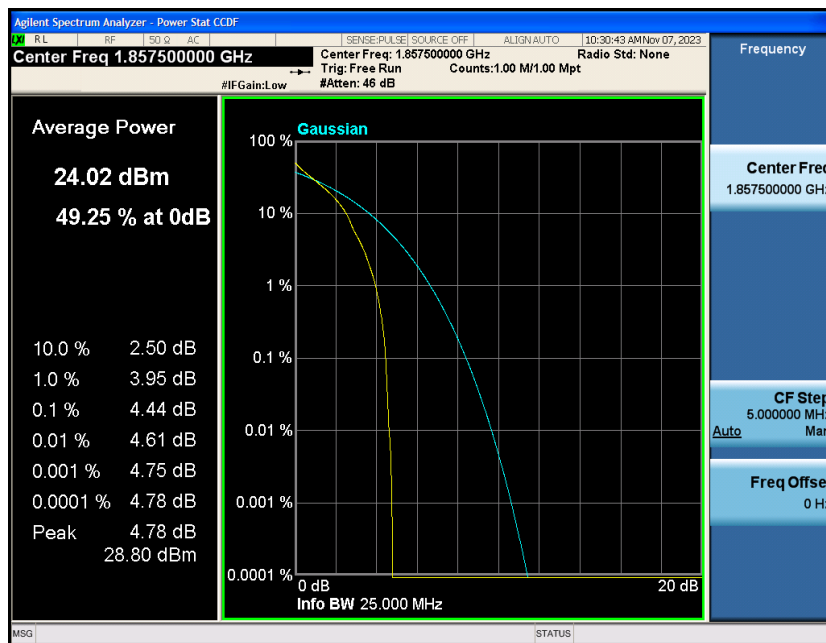
Band2-15MHz-QPSK-18675-75RB#0
