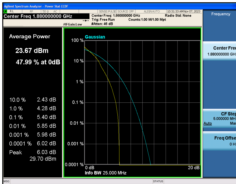
Band2-15MHz-QPSK-18900-75RB#0
