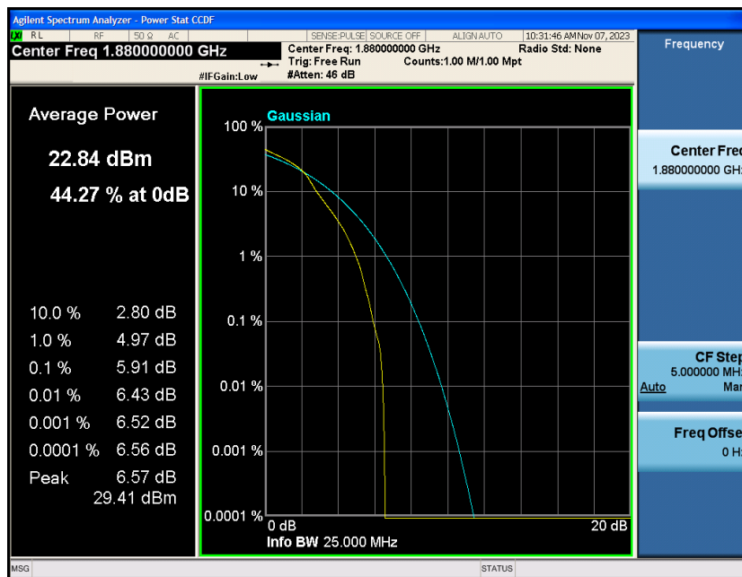
Band2-15MHz-16QAM-18900-75RB#0
