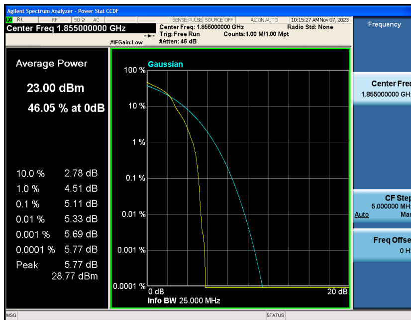
Band2-10MHz-16QAM-18650-50RB#0
