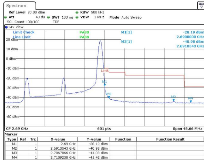
Band41-20MHz-QPSK-41490-100RB#0
