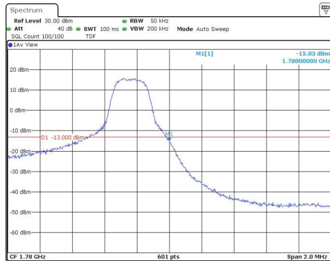
Band66-3MHz-QPSK-132657-15RB#0
