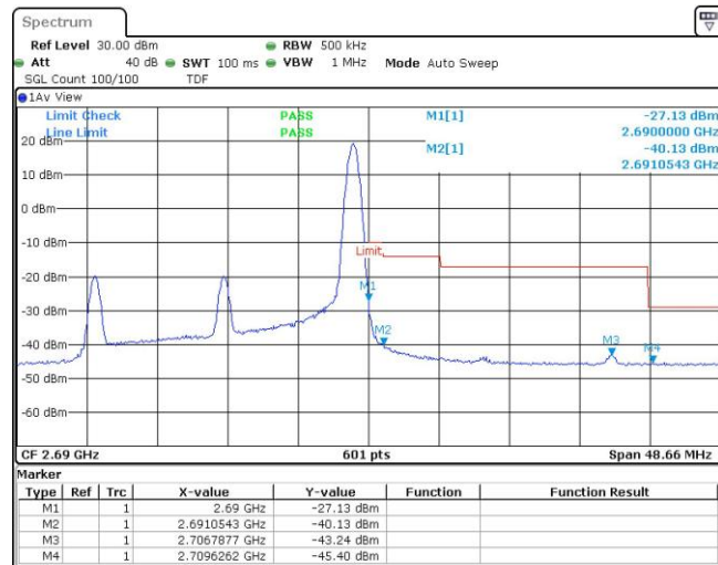
Band41-20MHz-16QAM-41490-100RB#0
