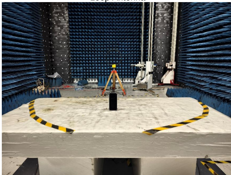
Loop Antenna
