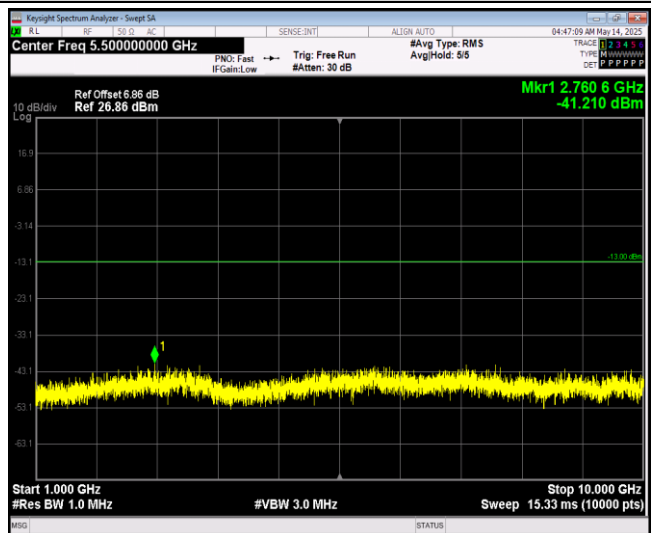
Band13-5MHz-64QAM-23230-1RB#0-Range2:1000~10000MHz
