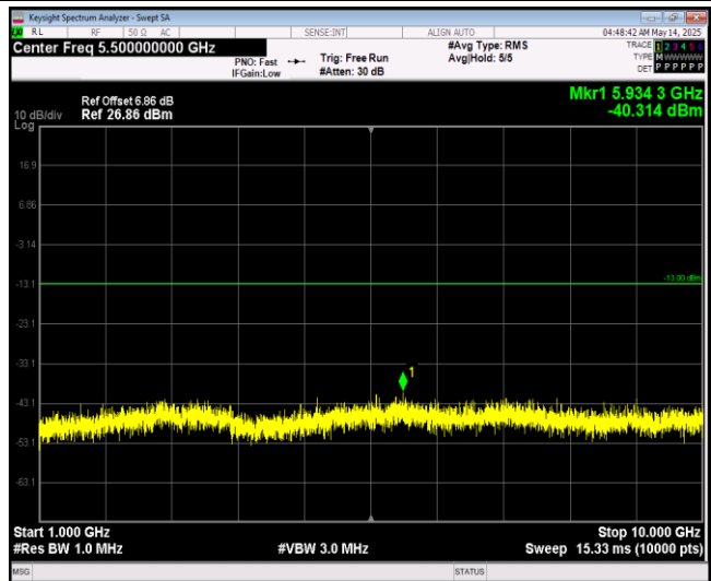
Band13-5MHz-64QAM-23205-1RB#0-Range2:1000~10000MHz
