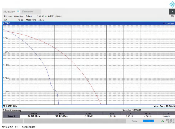
NTNV-n2-PC3-15-15-L-DFT-BPSK-Outer_Full-PASS
