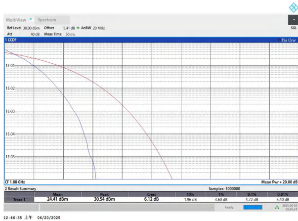
NTNV-n2-PC3-15-15-M-DFT-BPSK-Outer_Full-PASS
