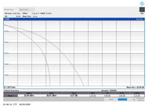
NTNV-n2-PC3-15-15-L-DFT-QPSK-Outer_Full-PASS
