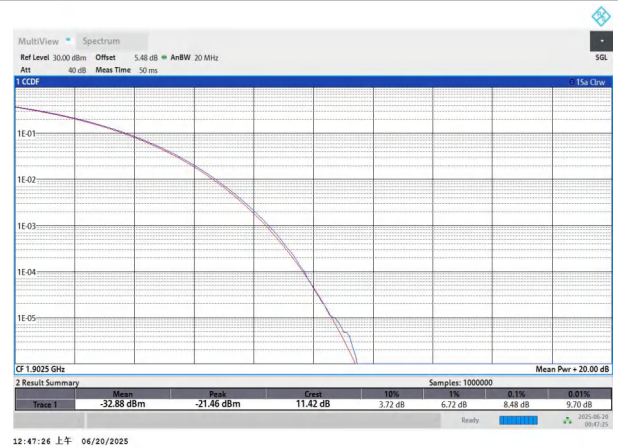
NTNV-n2-PC3-15-15-H-DFT-QPSK-Outer_Full-PASS
