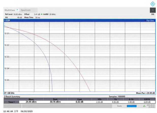
NTNV-n2-PC3-15-15-M-DFT-QPSK-Outer_Full-PASS
