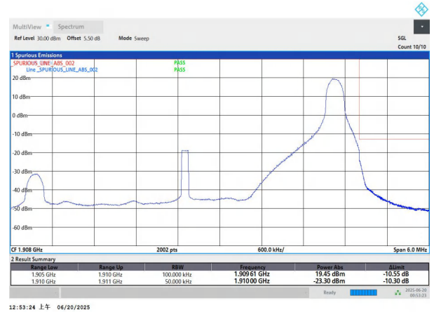
NTNV-n2-PC3-15-5-H-DFT-BPSK-Edge_1RB_Right-PASS
